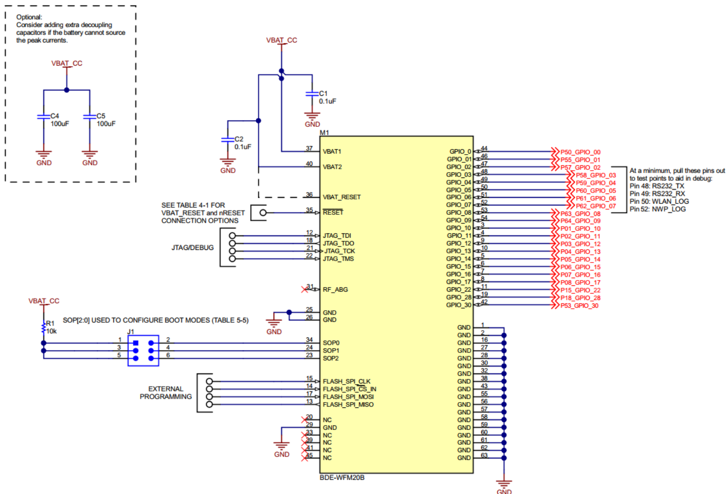
Figure 6-2. BDE-WFM20B Typical Application Schematic
