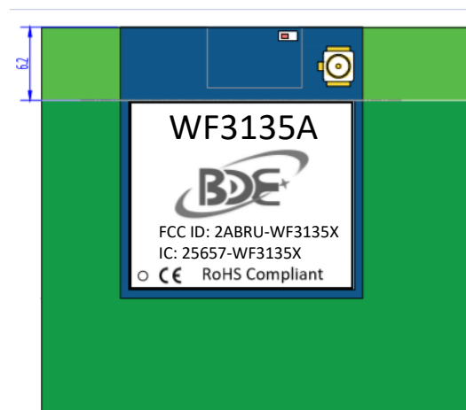
Figure 19. WF3135A Layout Guidelines
