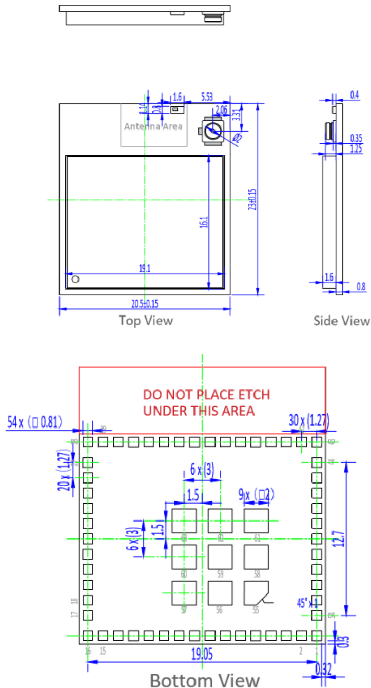
Figure 14. Mechanical Drawing
