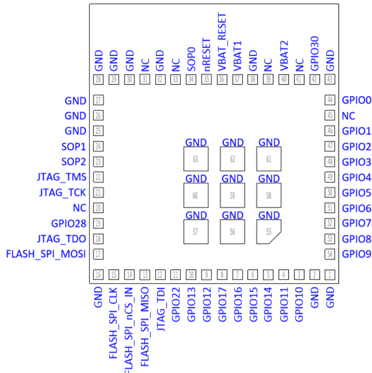
Figure 4. Pin Diagram Bottom View
