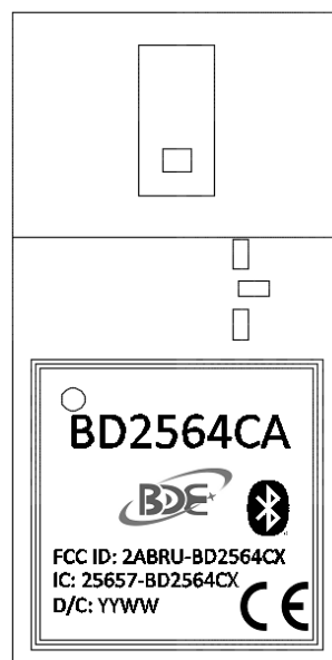
Figure 5-1. Module Marking
