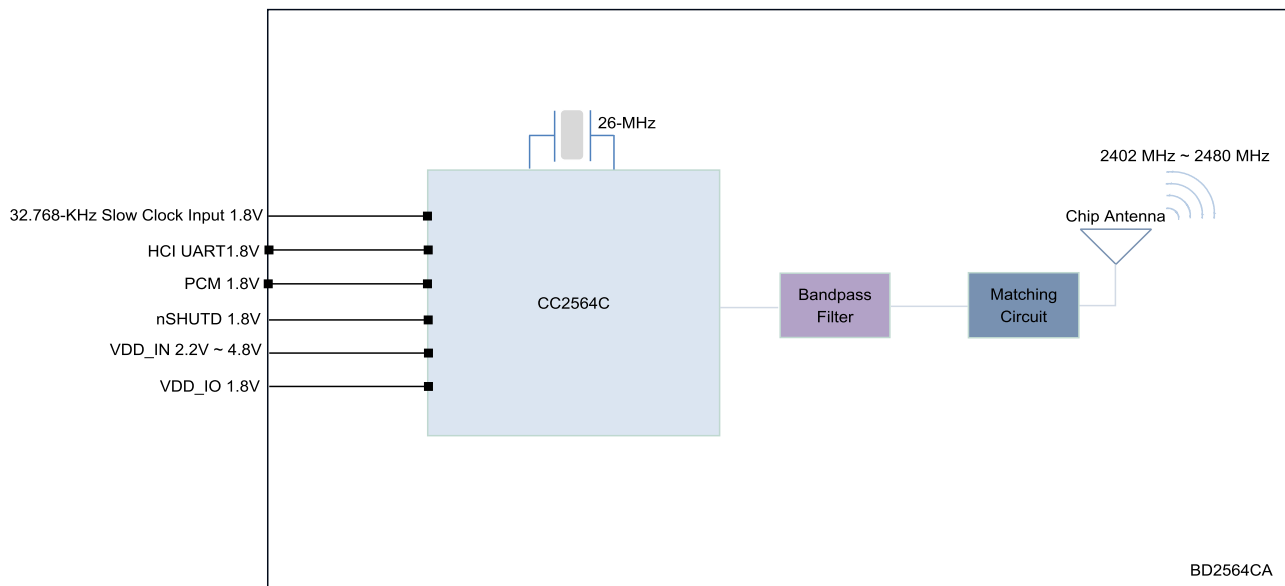
Figure 1-1. The block diagram of BD2564CA
