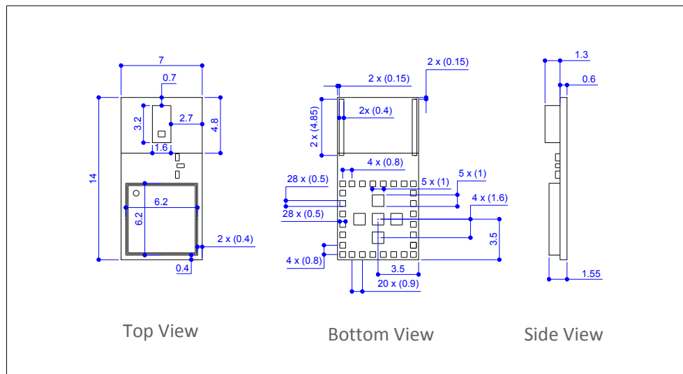
Figure 4-1. Mechanical Drawing
