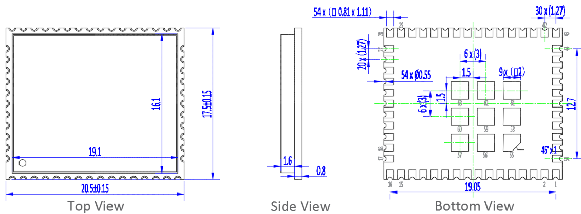
Figure 7-1: Mechanical Drawing
