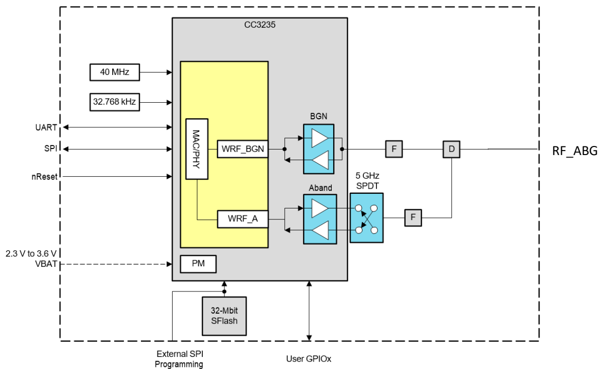
Figure 2-1. WF3235 Module Block Diagram
