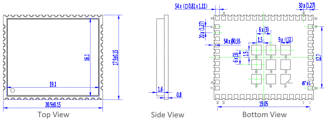
Figure 7-1: Mechanical Drawing
