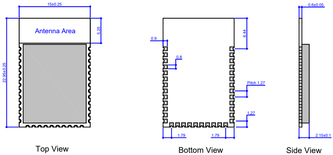
Fig 5-1. Mechanical Drawing
