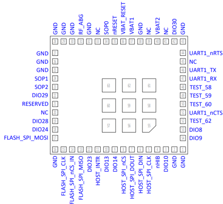
Pin Diagram Bottom View
