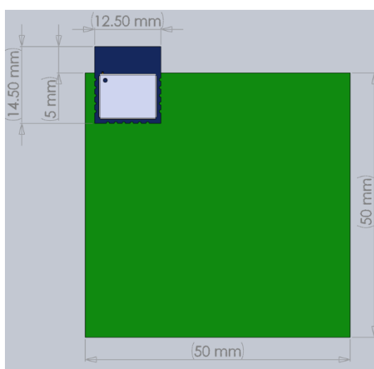
Figure 9: Mounting Positions for Optimum Antenna Performance
