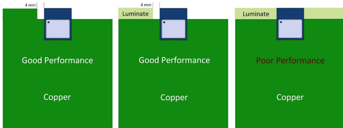
Figure 10: Antenna Performance Proximity with Copper (Left), Laminate (Middle) and Laminate Under Antenna (Right)
