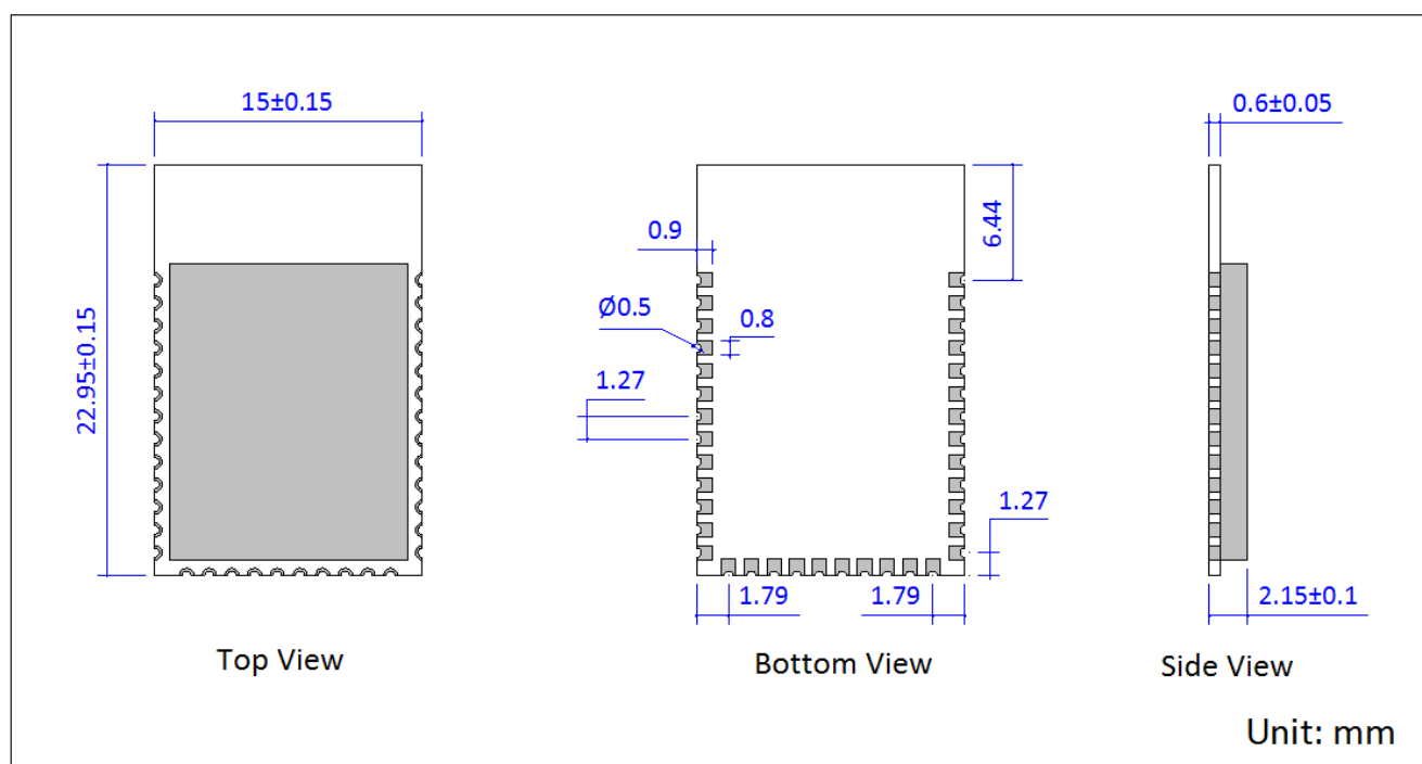
Figure 7-1. Mechanical Drawing
