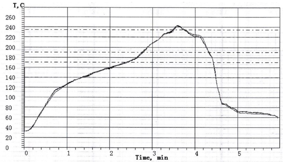
Fig 6-1. Typical Solder Reflow Profile
