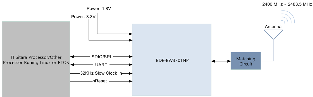
Figure 6-1. High-Level System Block Diagram
