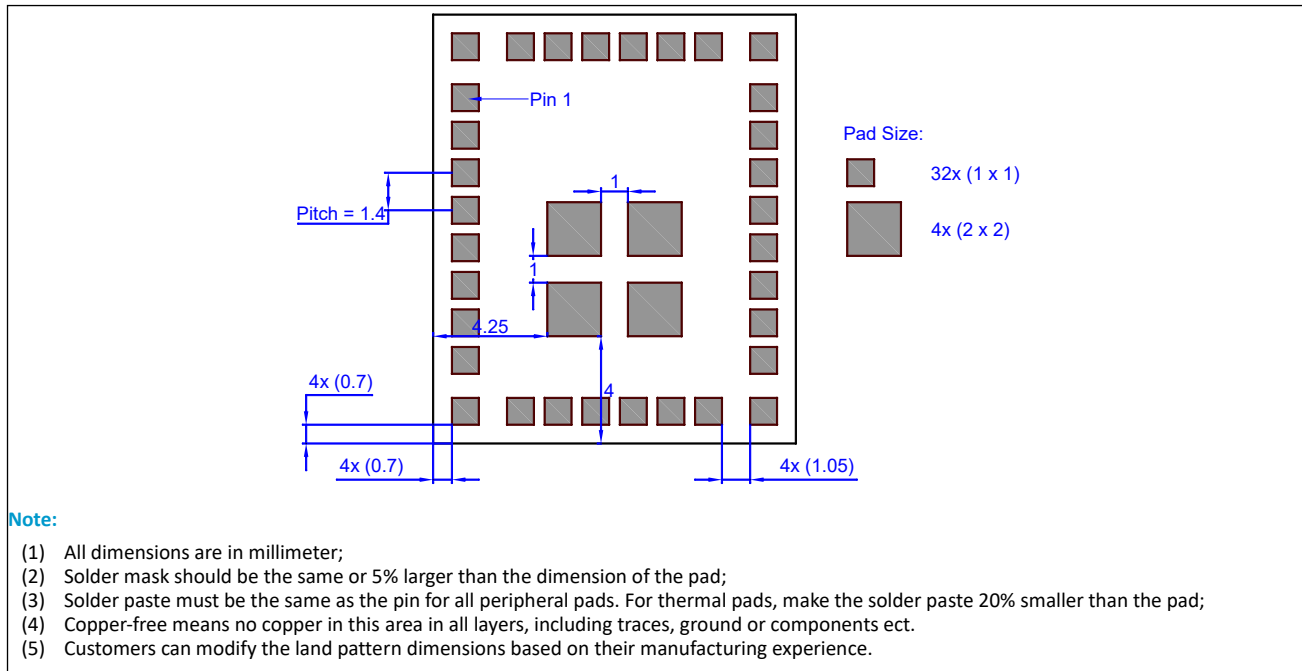
Figure 10. Module Footprint for BDE-HWF7394PN Top View
