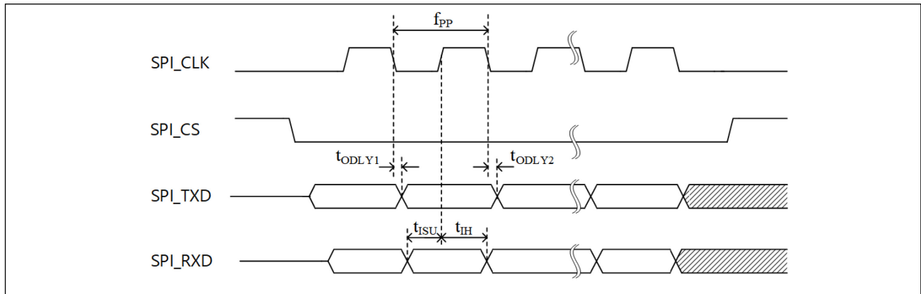
Figure 5. Timing Diagram of SPI
