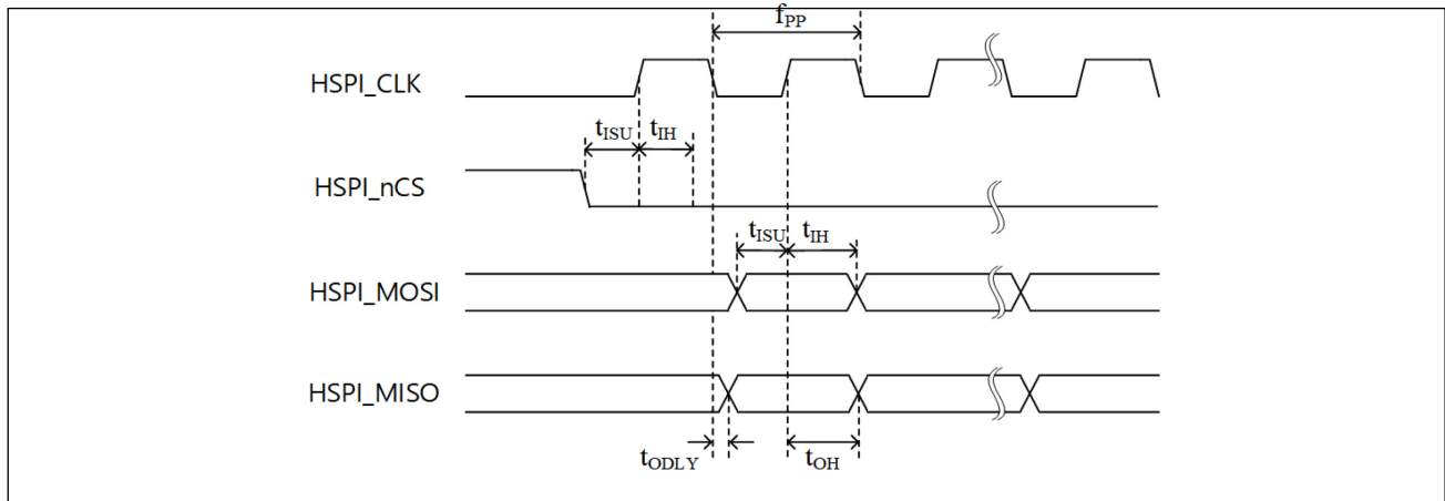
Figure 4. Timing Diagram of HSPI
