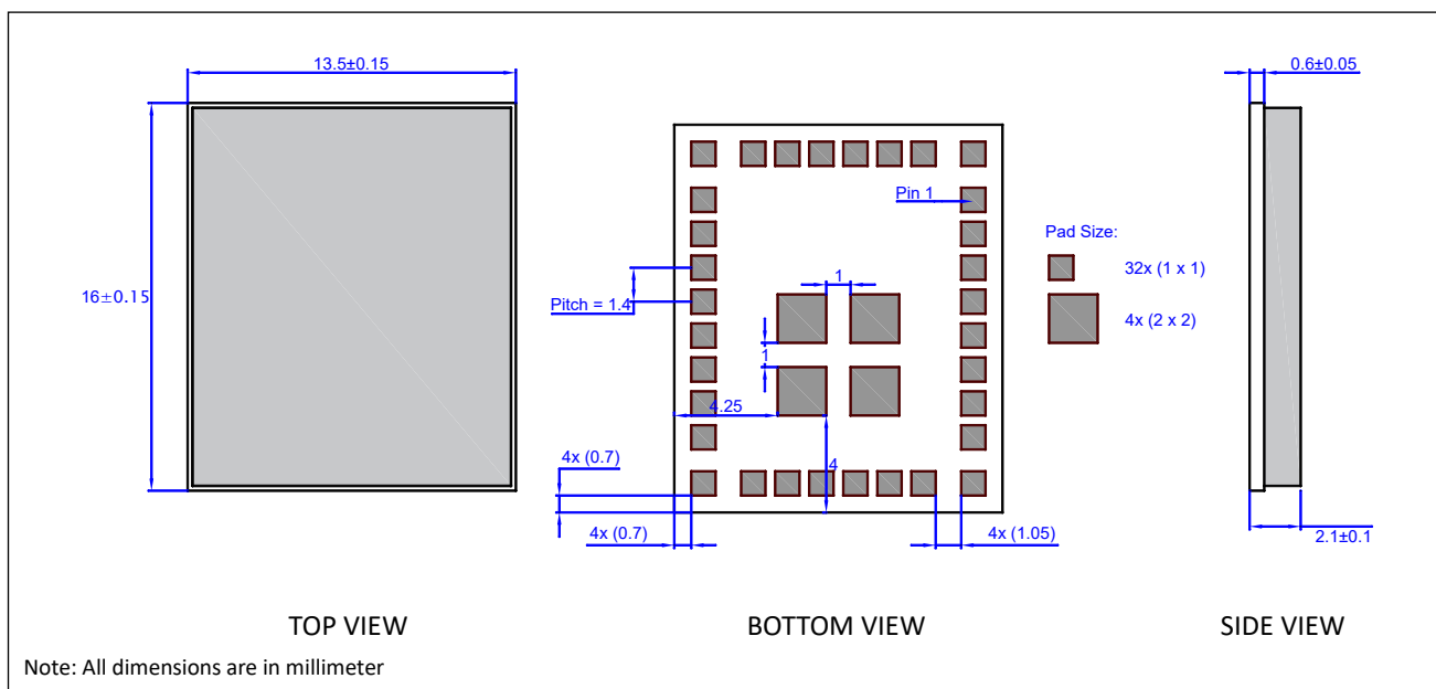
Figure 9. Mechanical Drawing for BDE-HWF7394PN
