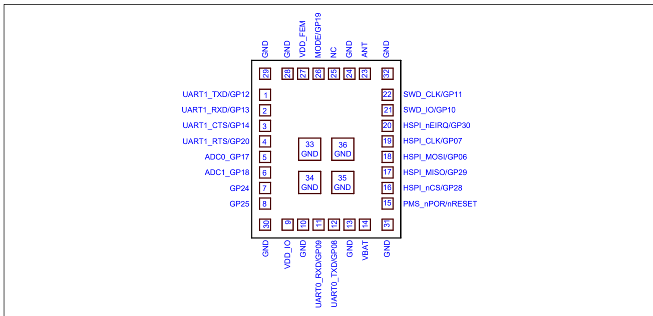
Figure 2. Pinout Diagram of BDE-HWF7394PN Top View
