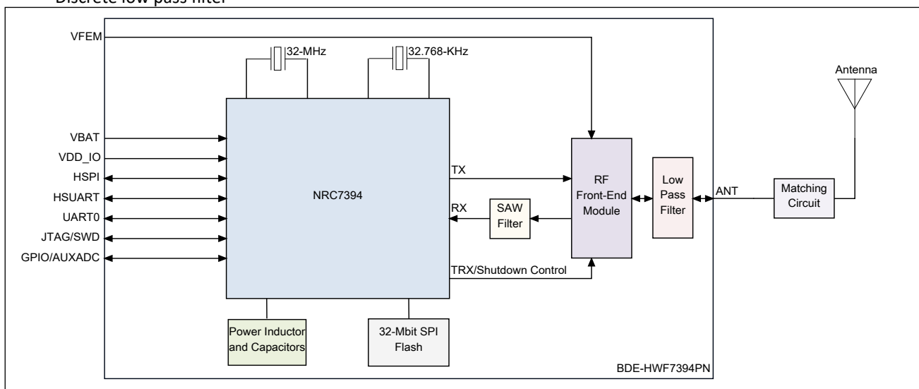
Figure 1. The Block Diagram of BDE-HWF7394PN
