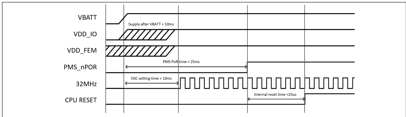
Figure 3. Power-On Sequence
