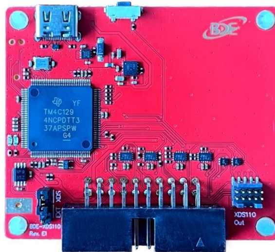
Figure 5. BDE-XDS110
