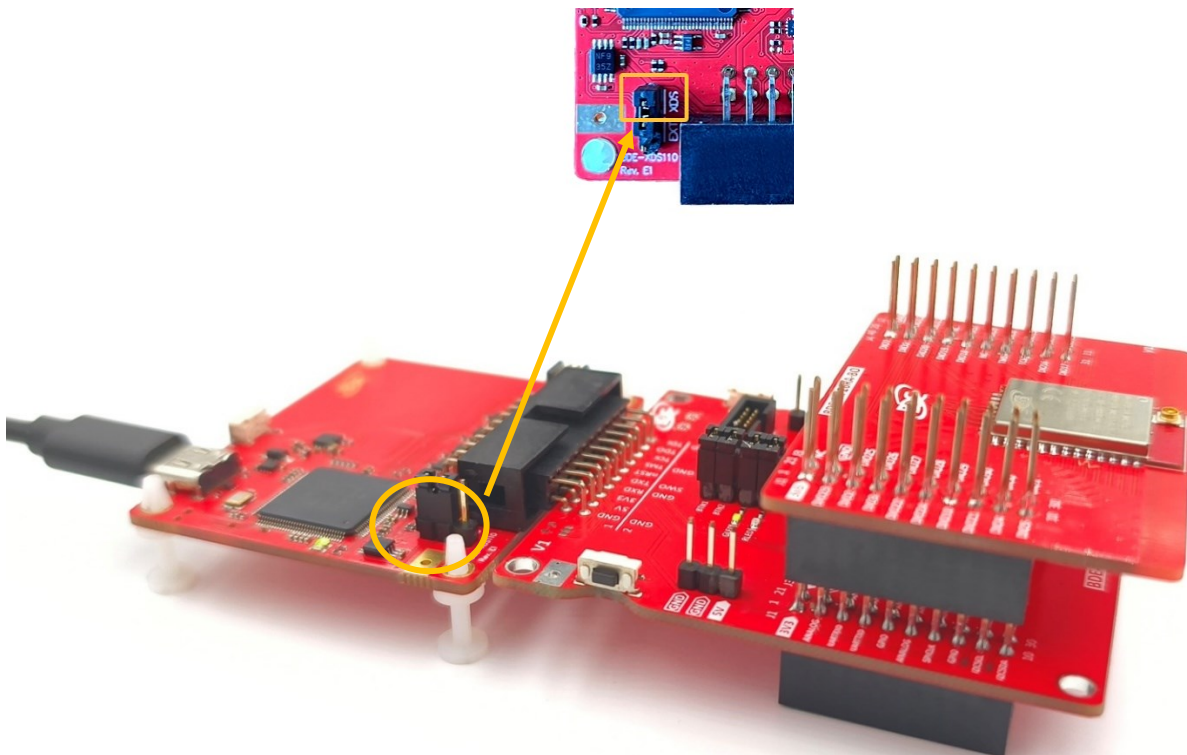
Figure 6. Hardware Setup
