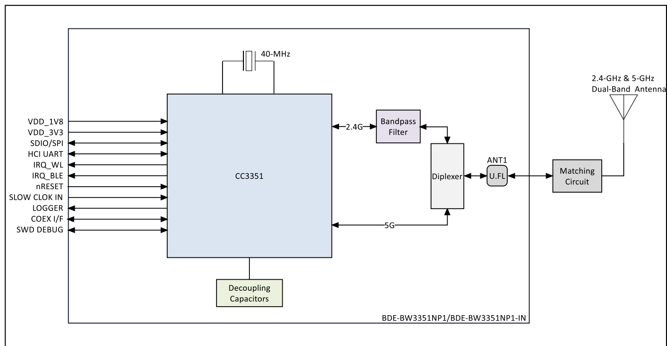
Figure 3. The Block Diagram of BDE-BW3351UP1 and BDE-BW3351UP1-IN
