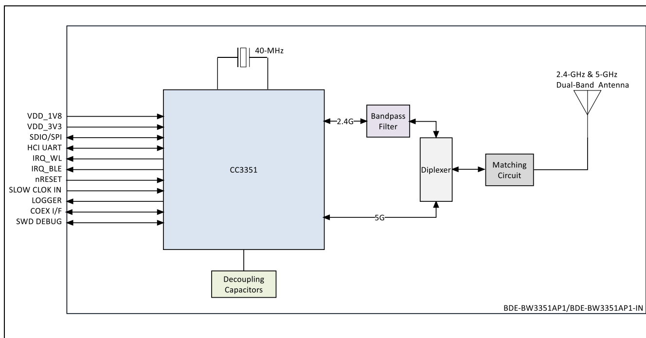
Figure 4. The Block Diagram of BDE-BW3351AP1 and BDE-BW3351AP1-IN
