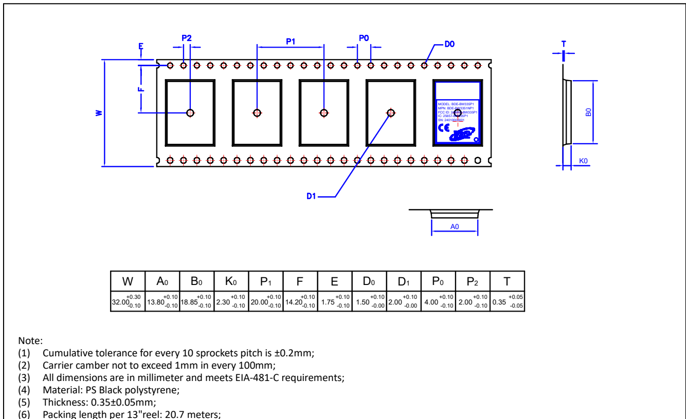
Figure 22. Carrier Tape Drawing for BDE-BW3351NP1 variants
