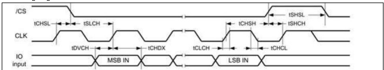
Figure 12. SPI Default Input Timing
