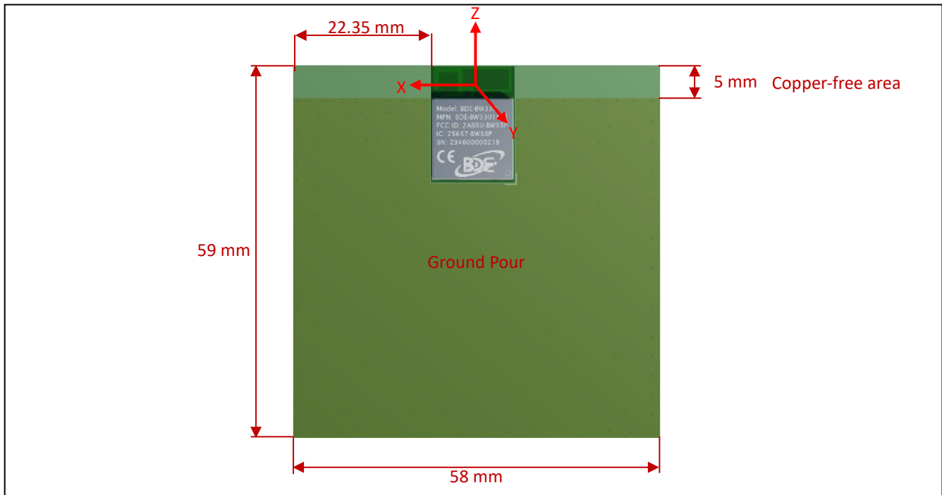
Figure 14. Antenna Placement and Reference Board
