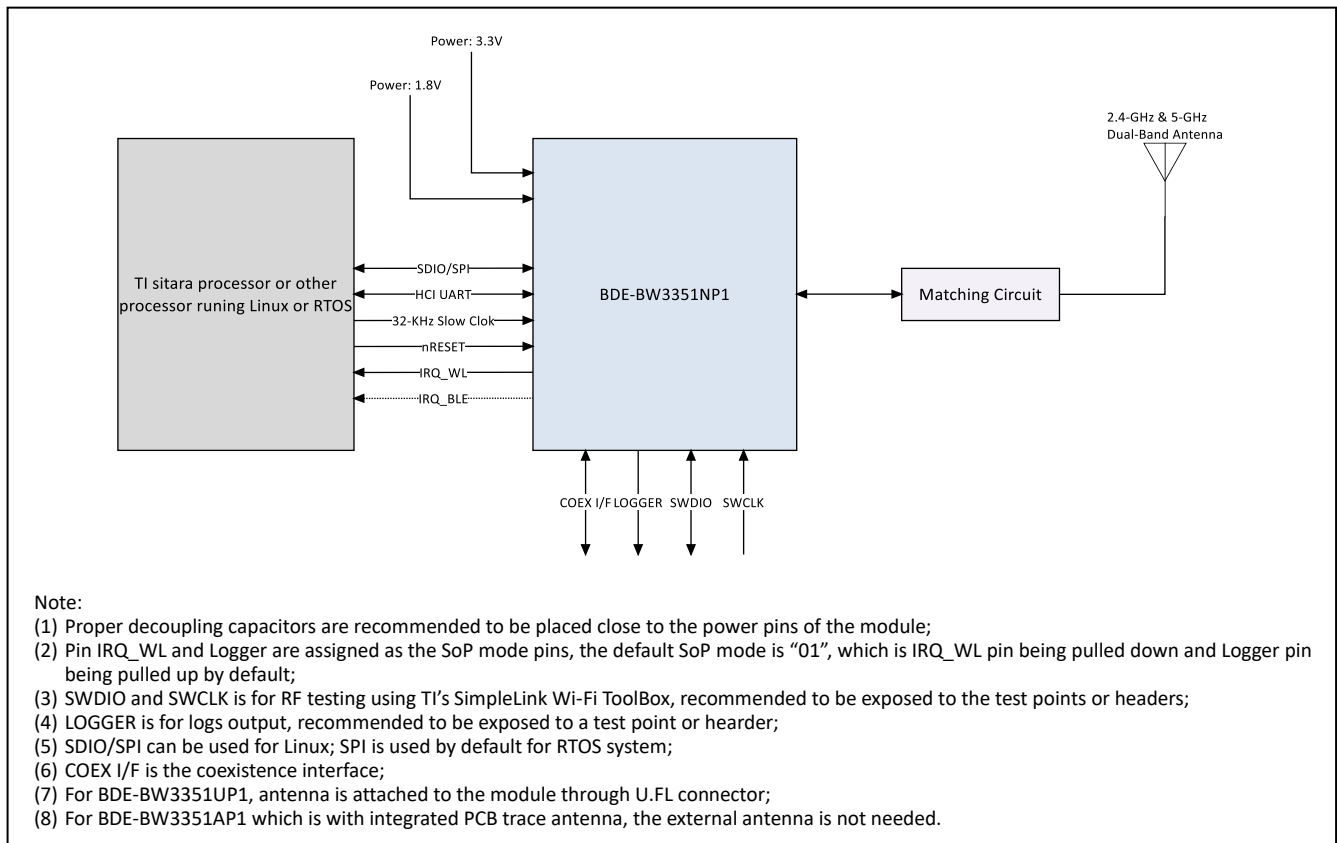
Figure 19. High-Level System Block Diagram
