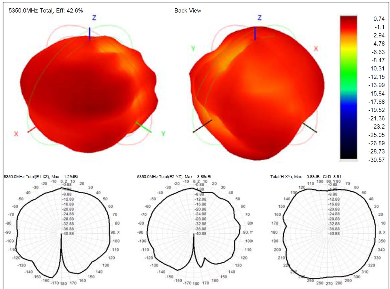
Figure 13. Radiation Pattern of the Integrated PCB Trace Antenna at 5530MHz
