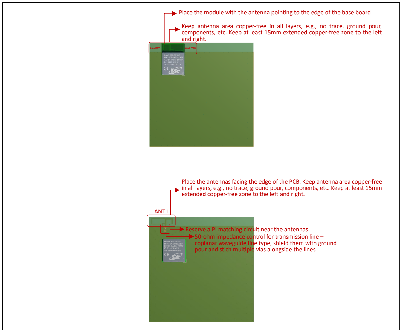
Figure 20. Recommended Module Placement
