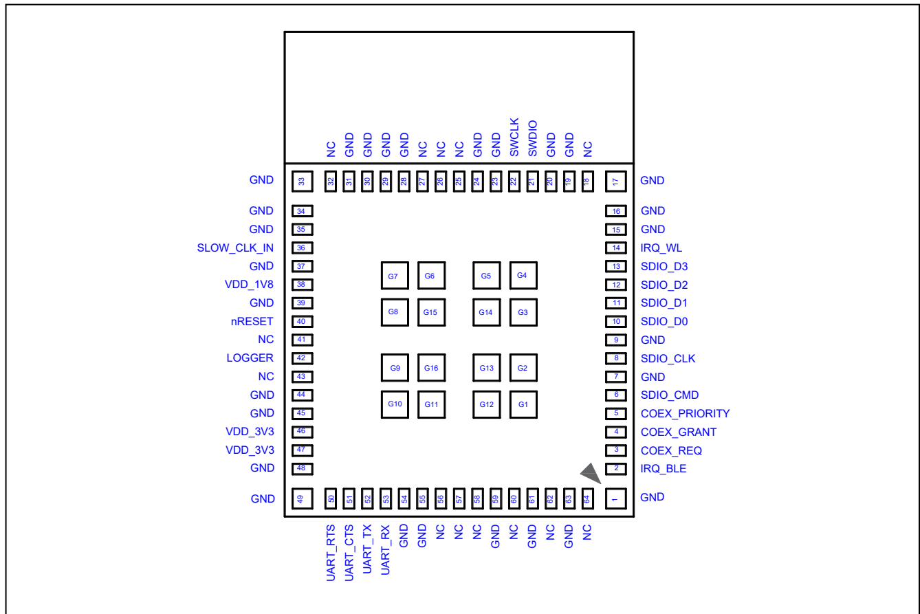
Figure 7. Pin Diagram of BDE-BW3351AP1 and BDE-BW3351UP1 (Top View)
