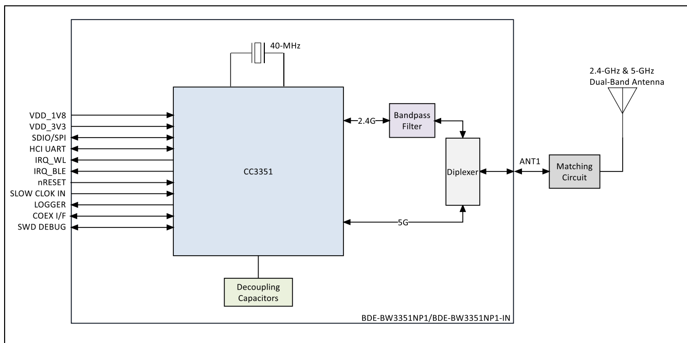
Figure 2. The Block Diagram of BDE-BW3351NP1 and BDE-BW3351NP1-IN
