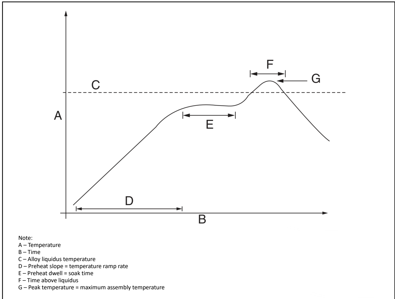
Figure 28. Thermal Profile Schematic
