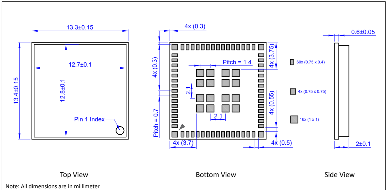
Figure 15. Mechanical Drawing of BDE-BW3351NP1
