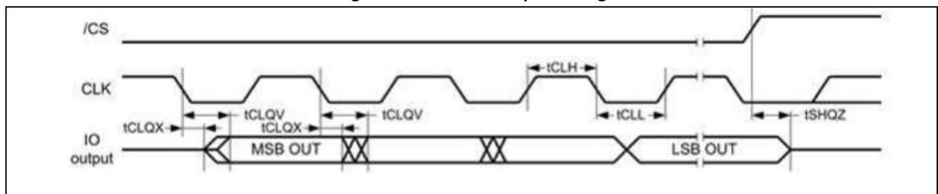
Figure 13. SPI Default Output Timing
