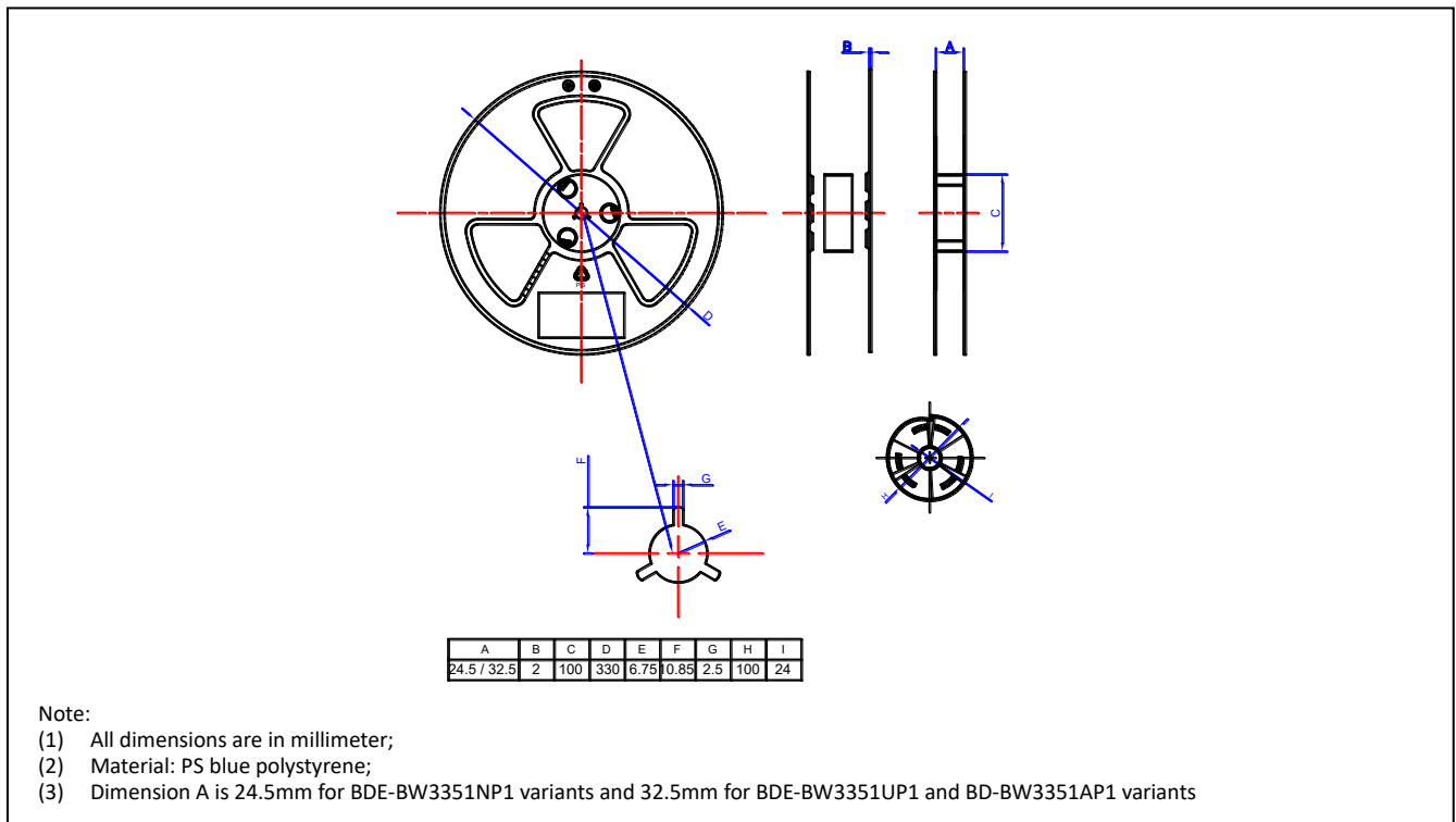
Figure 24. 13-Inch Reel Drawing
