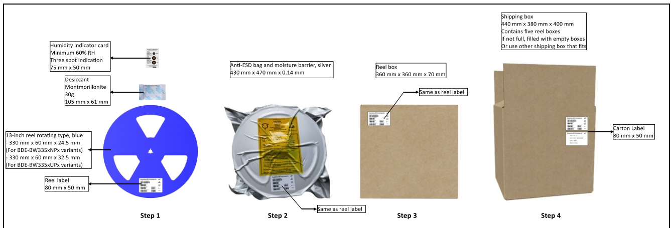
Figure 25. Carton Information
