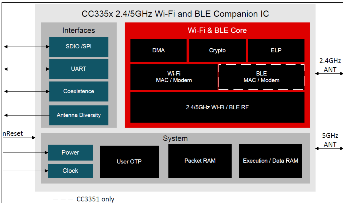
Figure 5. The Block Diagram of CC335x (Adopted form CC3351 Datasheet)
