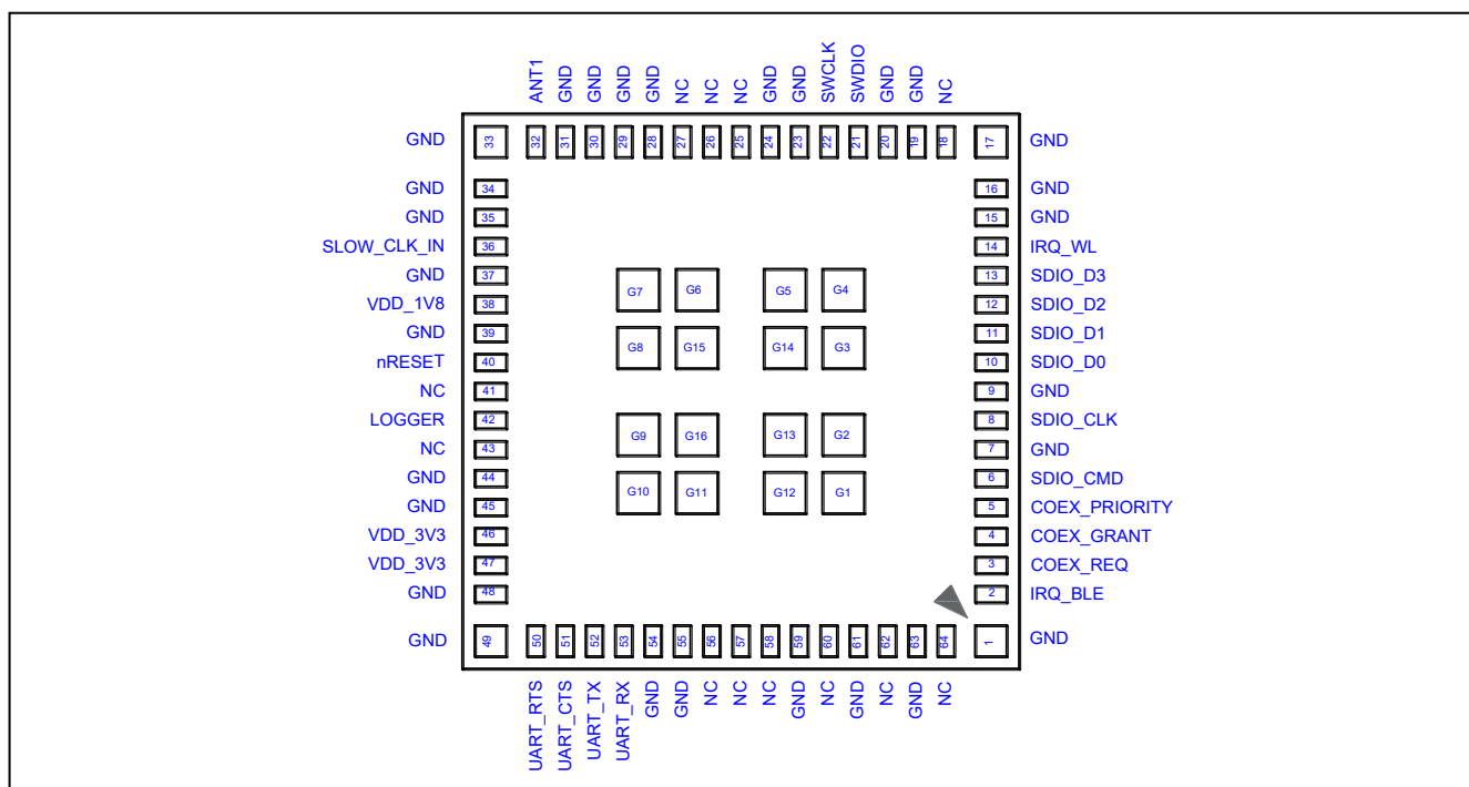
Figure 6. Pin Diagram of BDE-BW3351NP1 (Top View)
