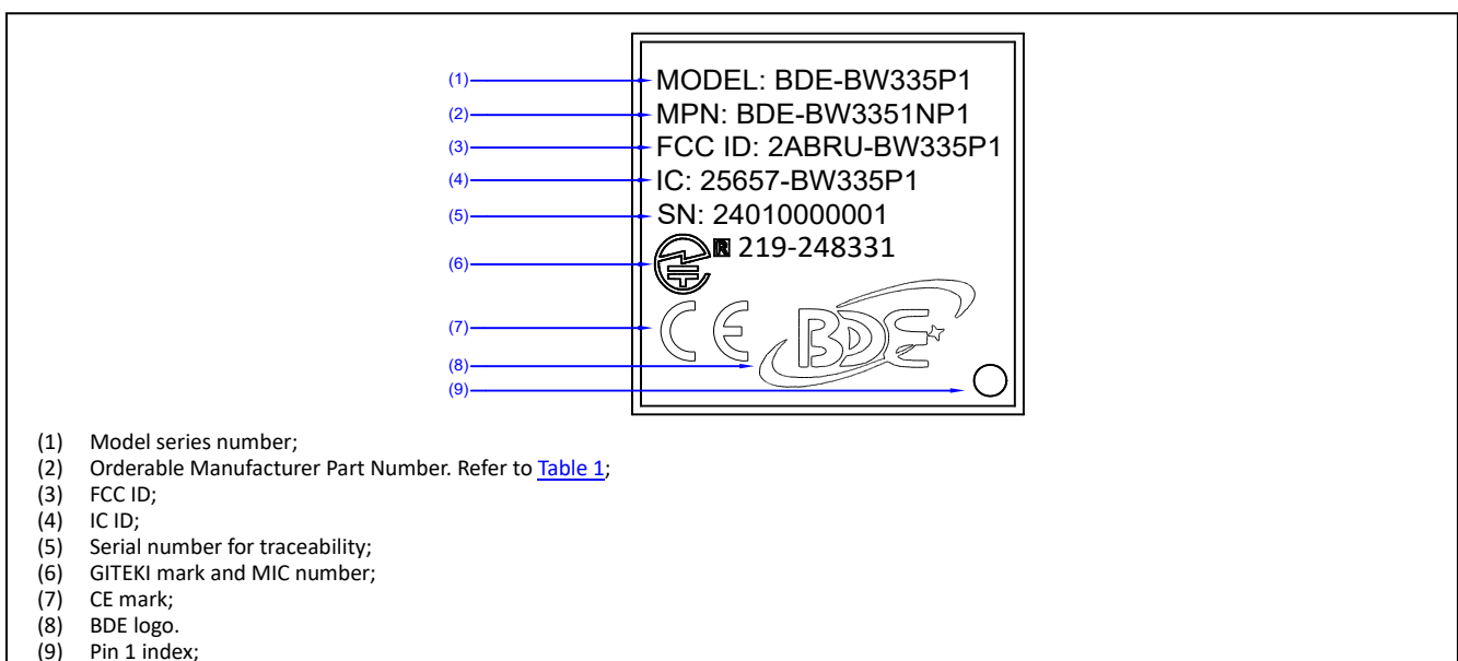
Figure 21. Module Marking
