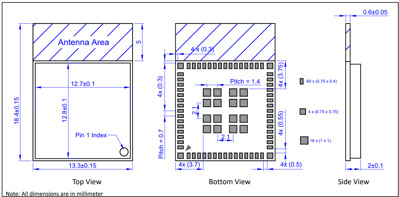
Figure 16. Mechanical Drawing of BDE-BW3351AP1 and BDE-BW3351UP1
