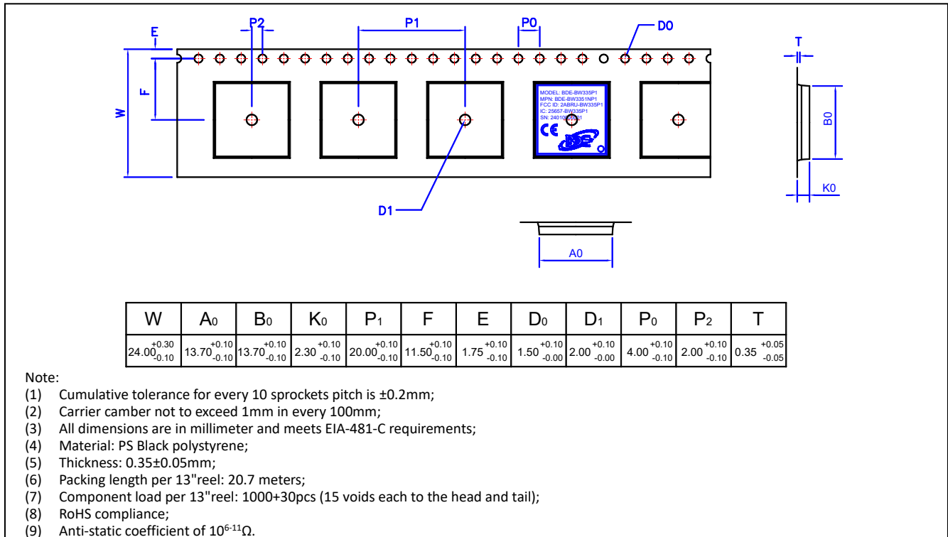
Figure 22. Carrier Tape Drawing for BDE-BW3351NP1 variants
