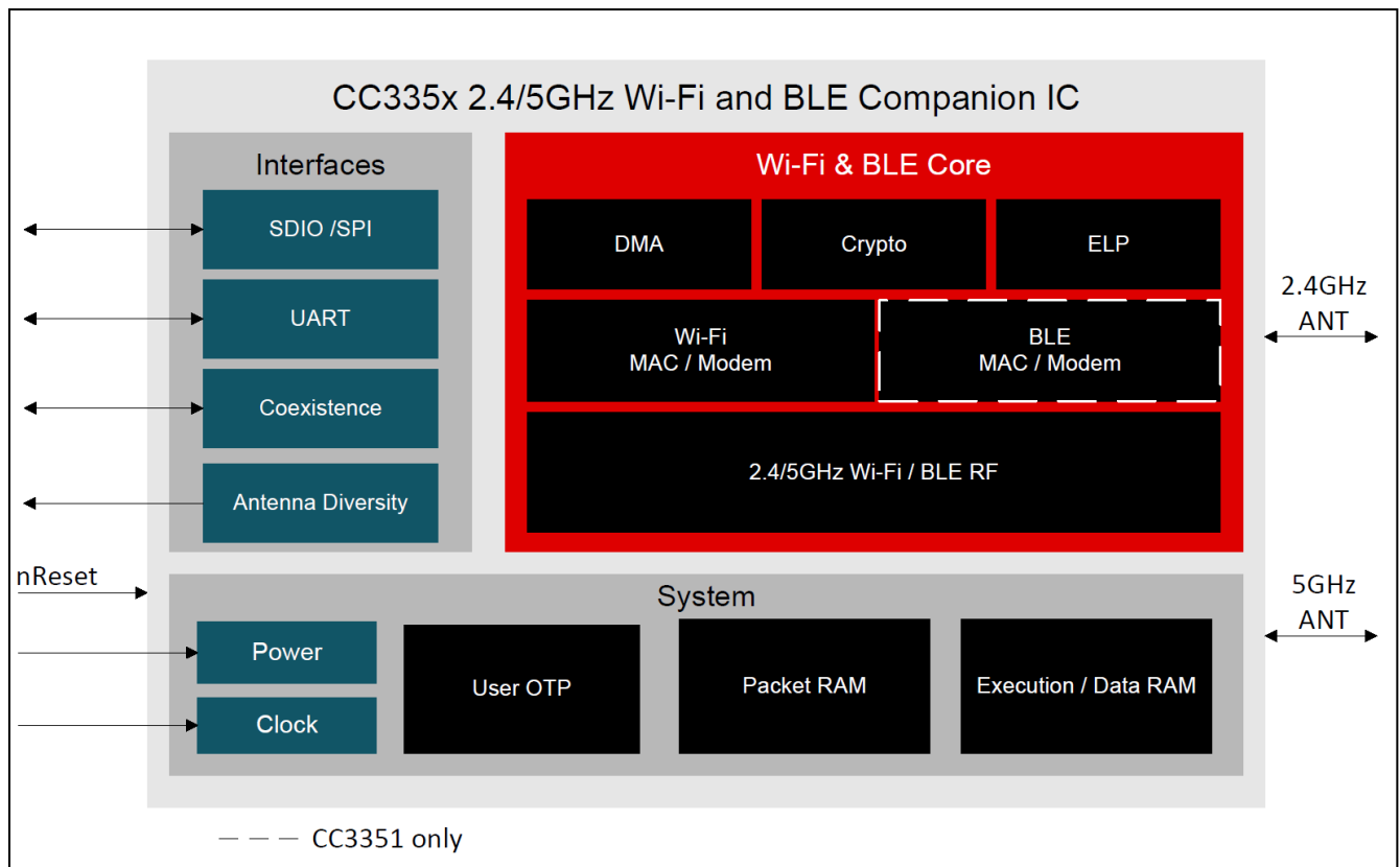
Figure 5. The Block Diagram of CC335x (Adopted form CC335x Datasheet)
