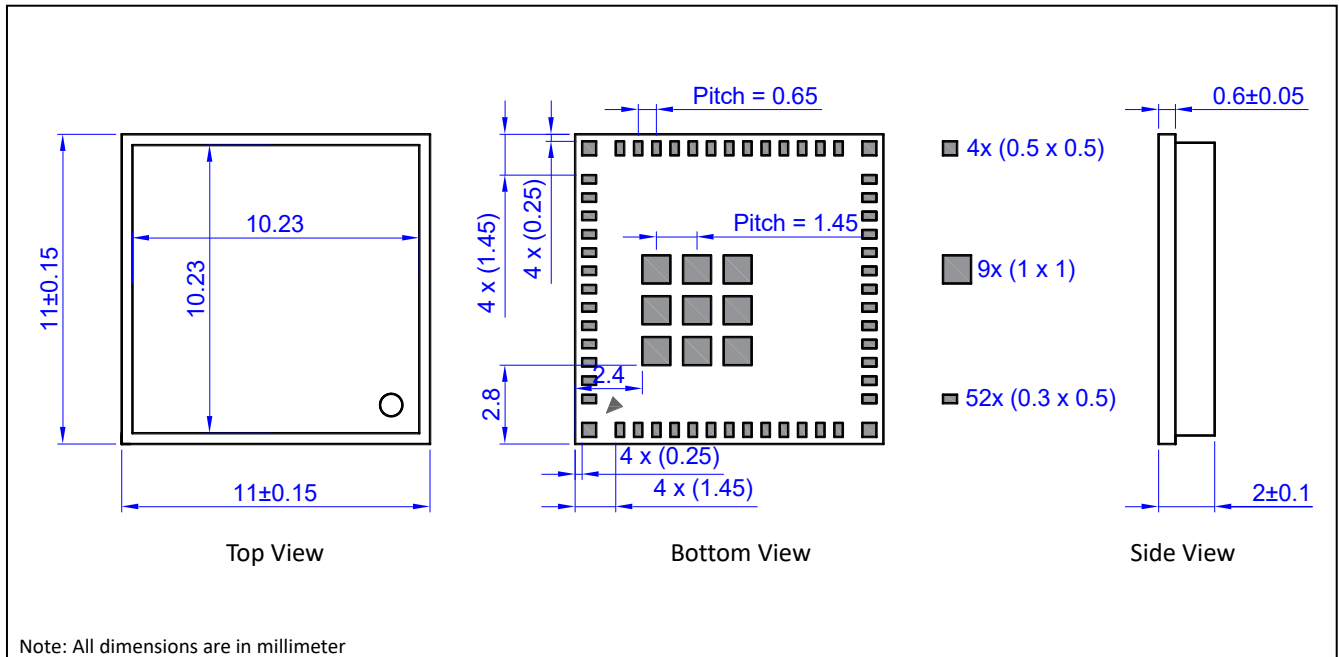
Figure 15. Mechanical Drawing of BDE-BW3351N1
