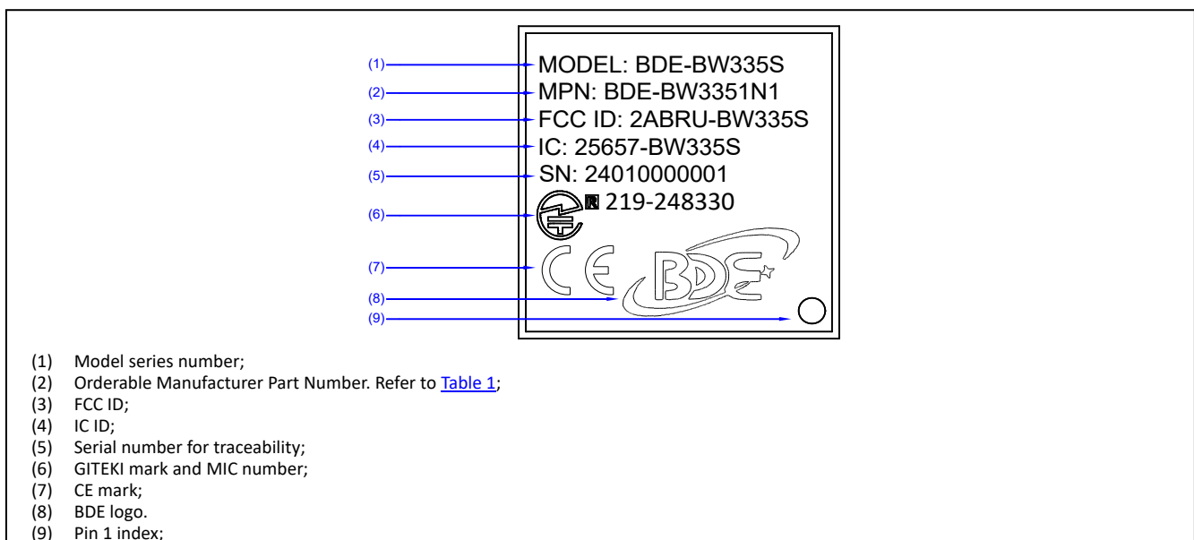
Figure 22. Module Marking
