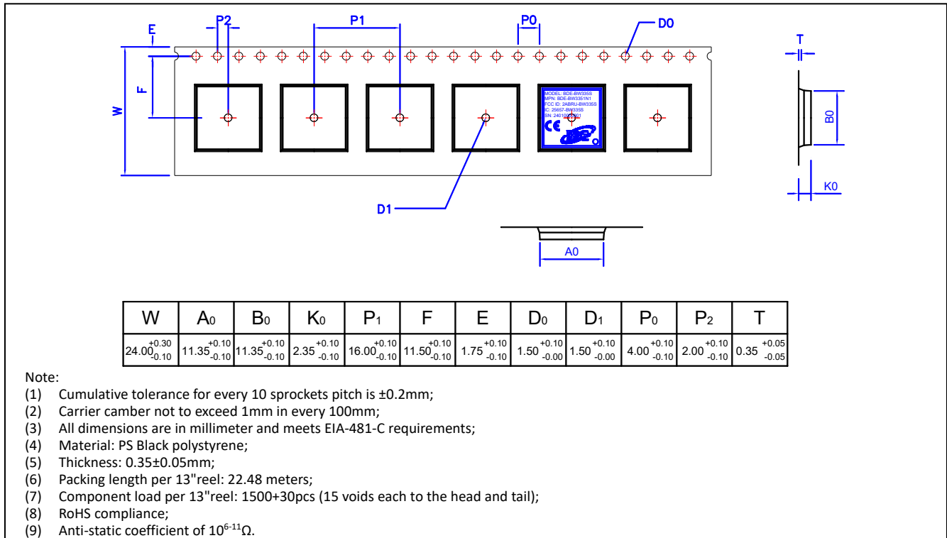
Figure 23. Carrier Tape Drawing for BDE-BW3351N1 Variants
