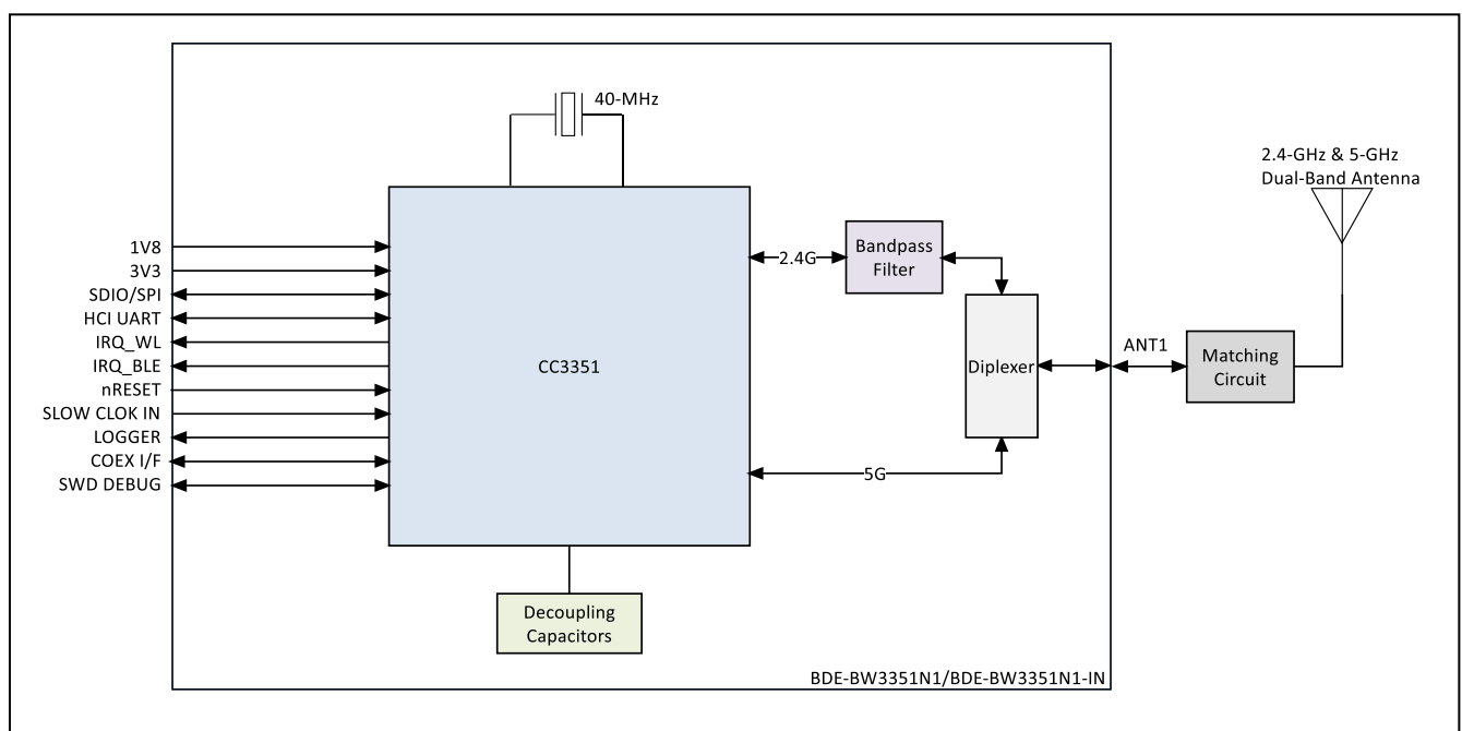
Figure 2. The Block Diagram of BDE-BW3351N1 and BDE-BW3351N1-IN
