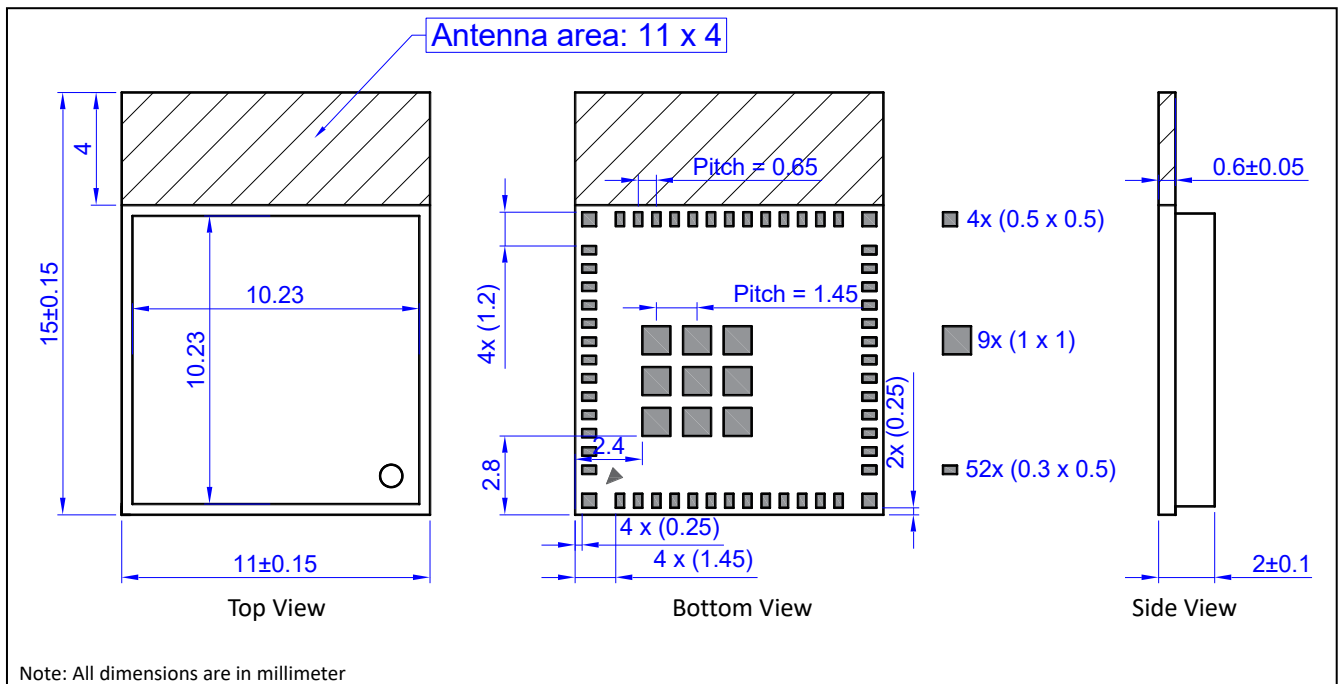
Figure 16. Mechanical Drawing of BDE-BW3351A1
