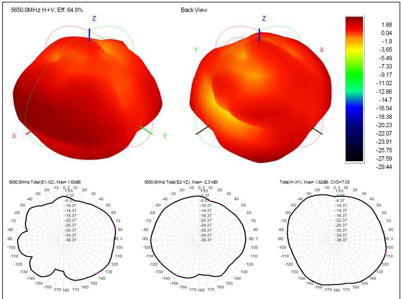
Figure 13. Radiation Pattern of the Integrated PCB Trace Antenna at 5650MHz
