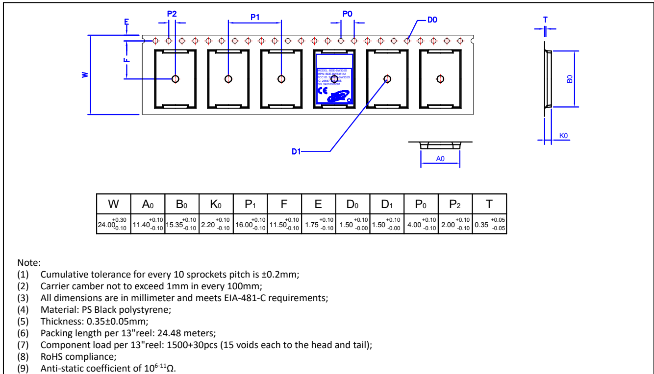
Figure 24. Carrier Tape Drawing for BDE-BW3351U1 and BDE-BW3351A1 Variants
