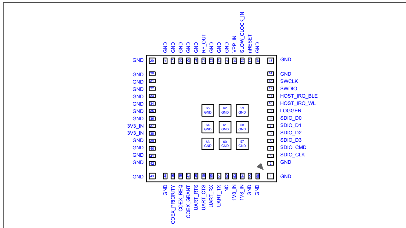
Figure 6. Pin Diagram of BDE-BW3351N1 (Top View)
