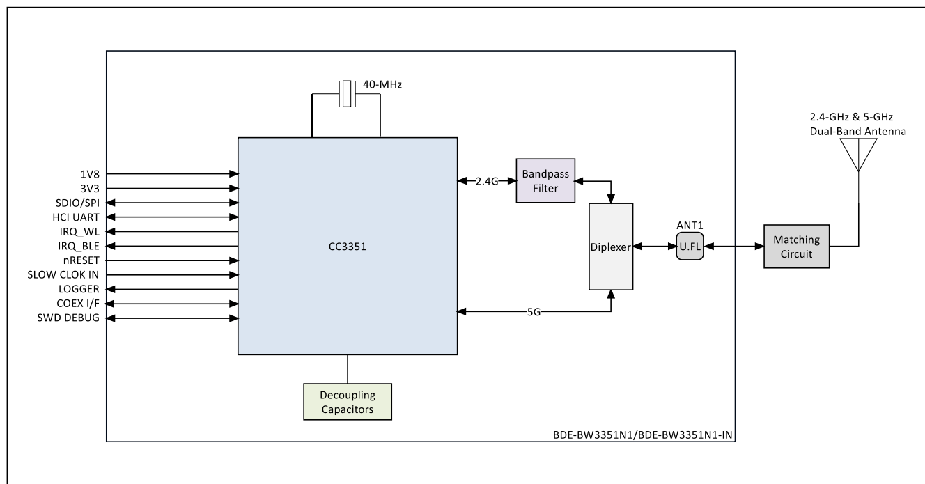
Figure 3. The Block Diagram of BDE-BW3351U1 and BDE-BW3351U1-IN
