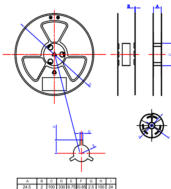
Figure 25. 13-Inch Reel Drawing
