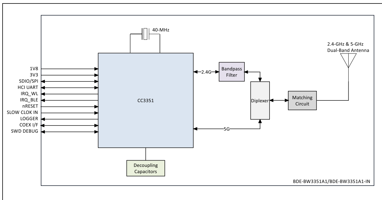
Figure 4. The Block Diagram of BDE-BW3351A1 and BDE-BW3351A1-IN
