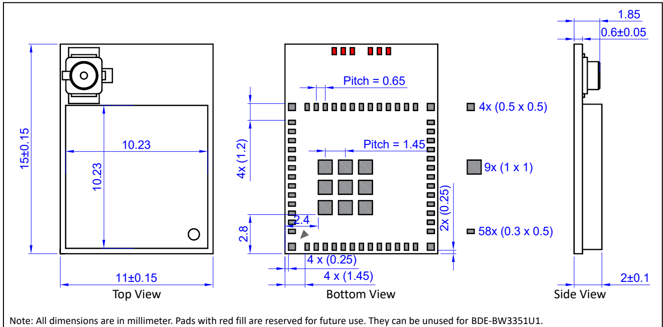
Figure 17. Mechanical Drawing of BDE-BW3351U1
