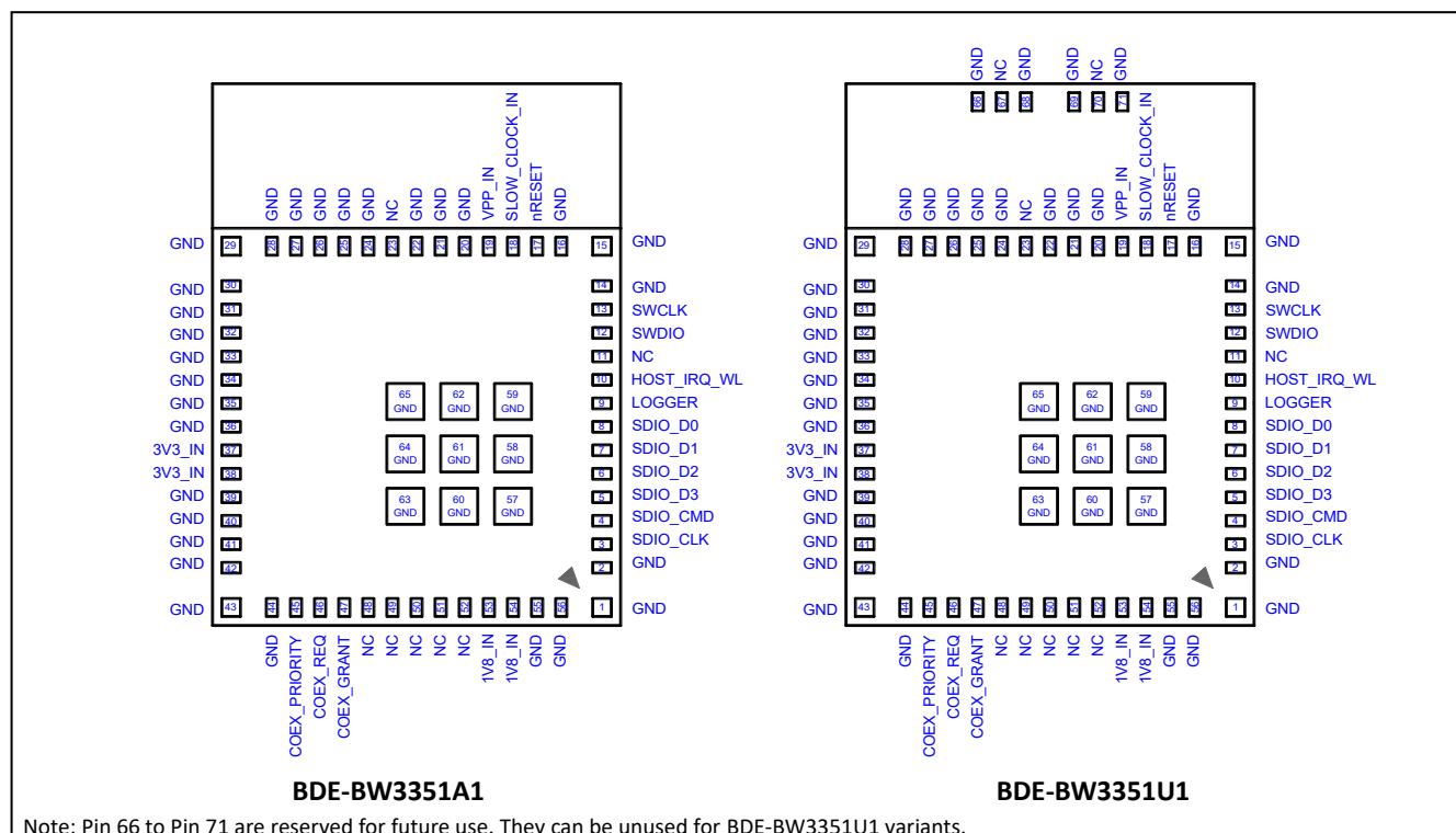
Figure 7. Pin Diagram of BDE-BW3351A1 (Top View)
