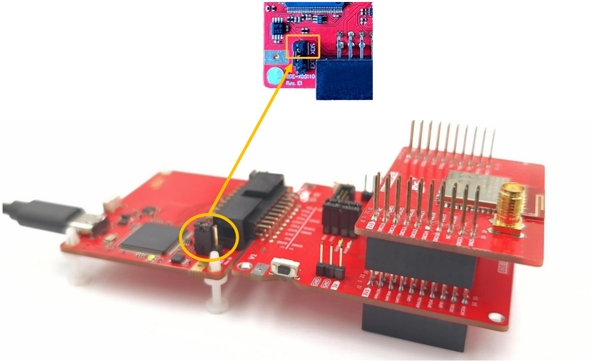
Figure 6. Hardware Setup
