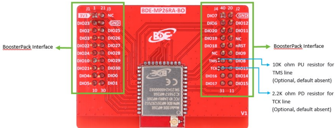
Figure 2. Board Overview of BDE-MP26RA-BO
