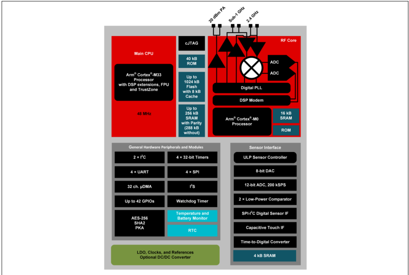
Figure 3. The block diagram of CC1354P10 (Adopted from CC1354P10 Datasheet)
