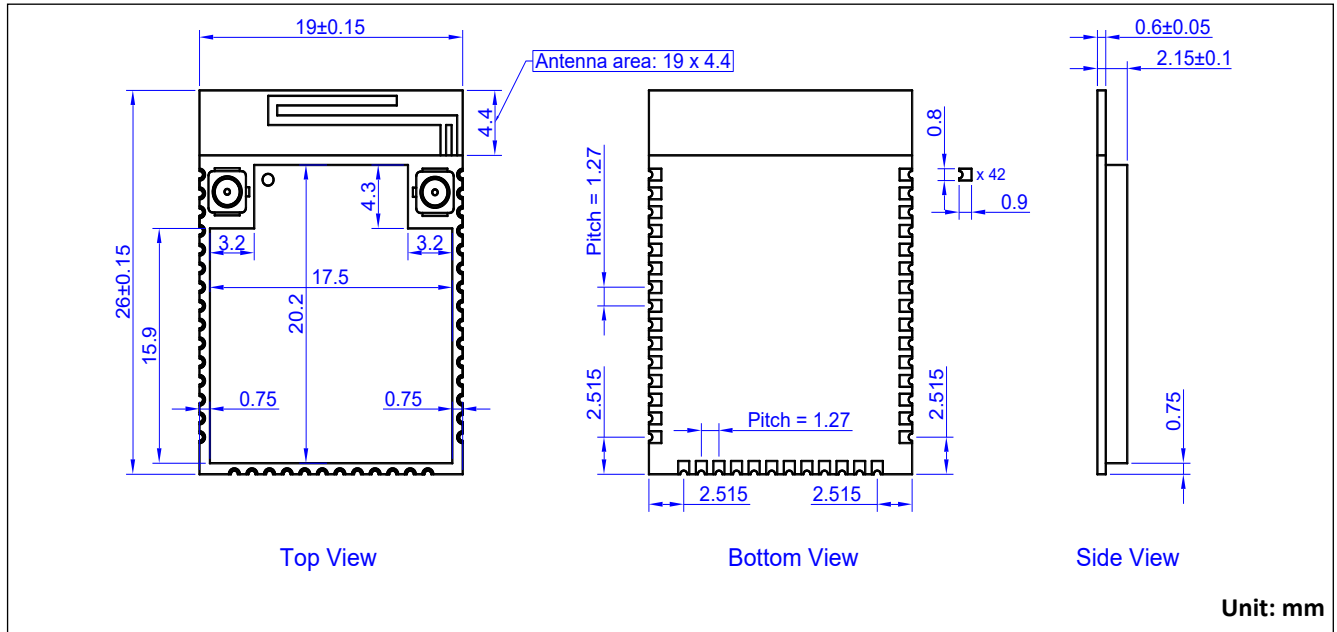
Figure 7. Mechanical Drawing of BDE-MB1354P102
