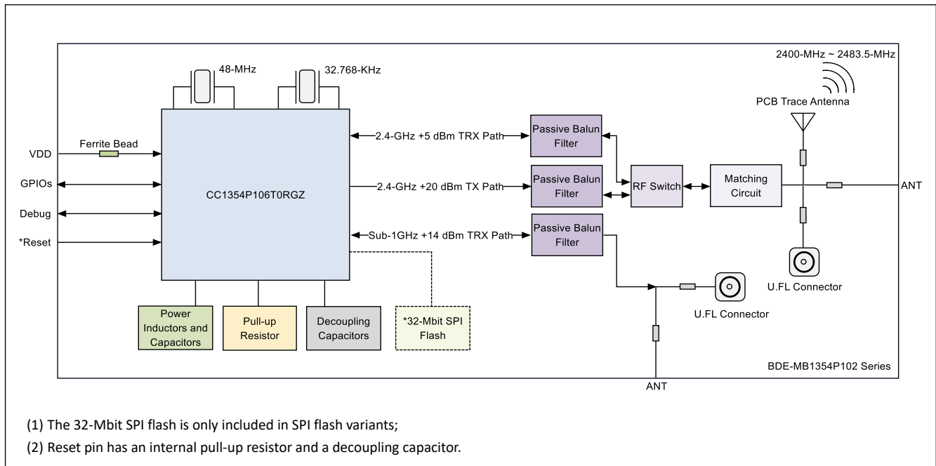
Figure 2. BDE-MB1354P102 Module Block Diagram
