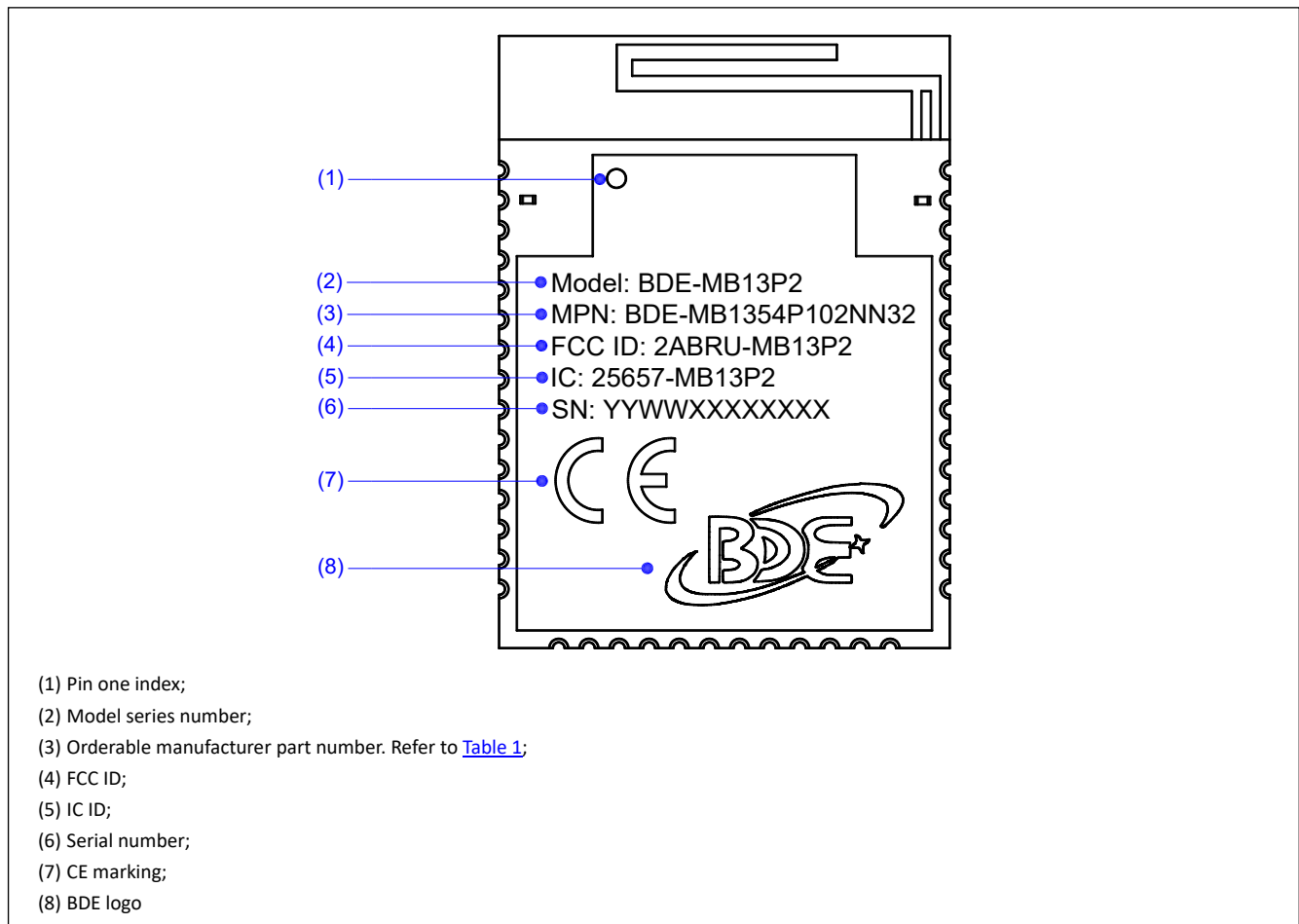
Figure 12. Module Marking
