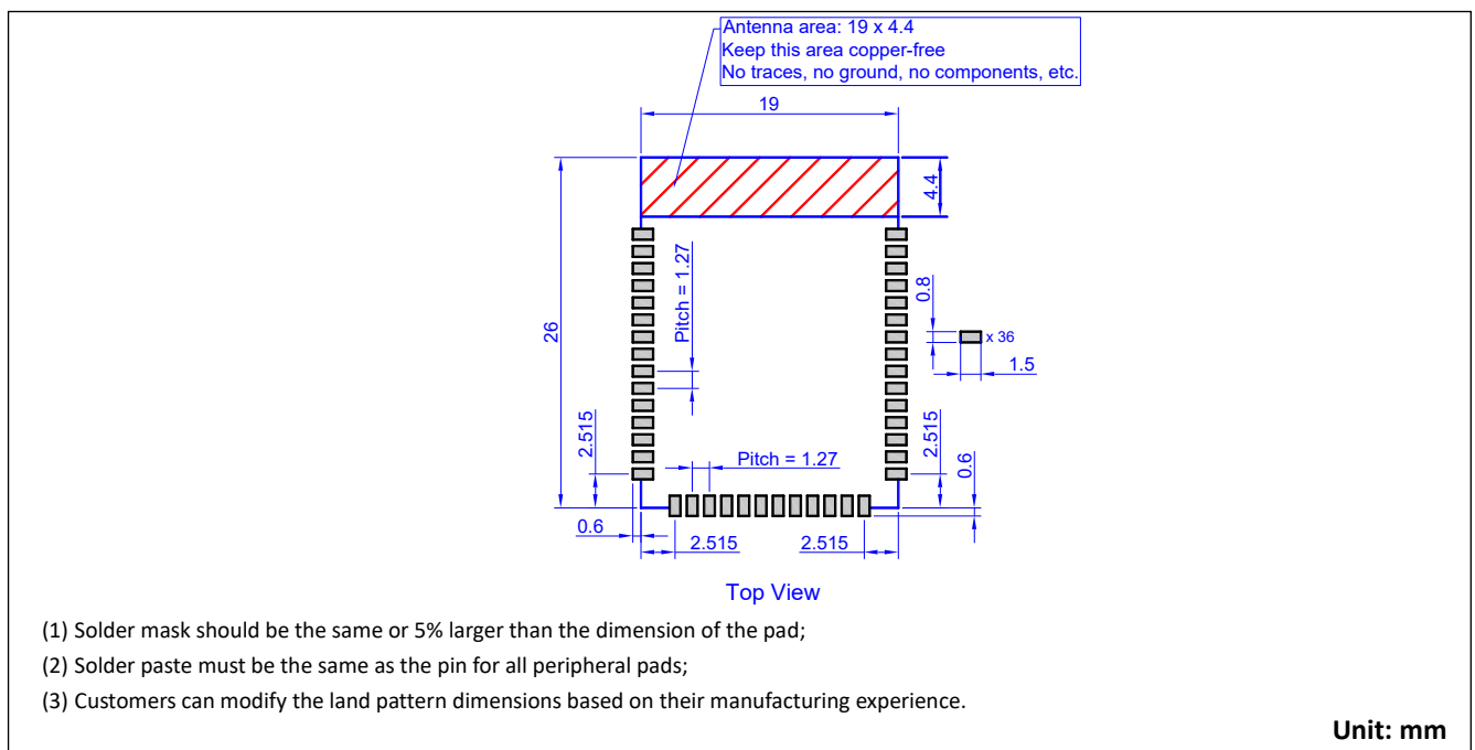
Figure 8. Recommended Module Footprint of BDE-MB1354P102
