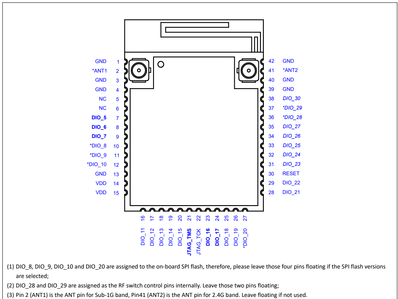
Figure 4. Pin Diagram of BDE-MB1354P102 (Top View)
