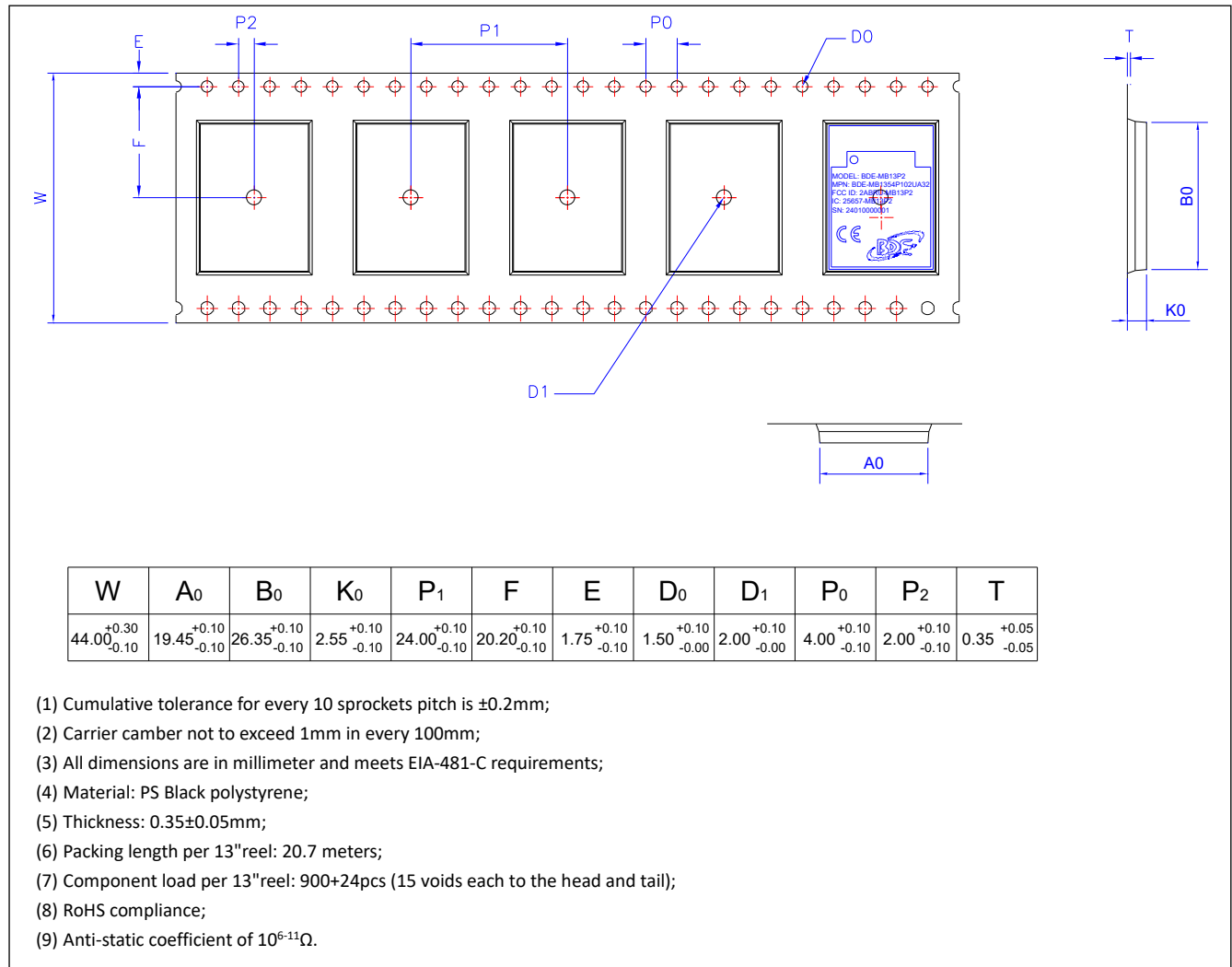
Figure 13. Carrier Tape Drawing for BDE-MB1354P102 variants
