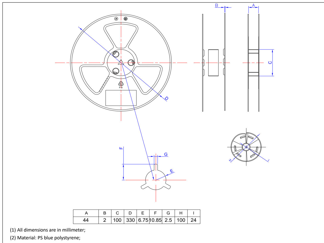
Figure 14. 13-INch Reel Drawing
