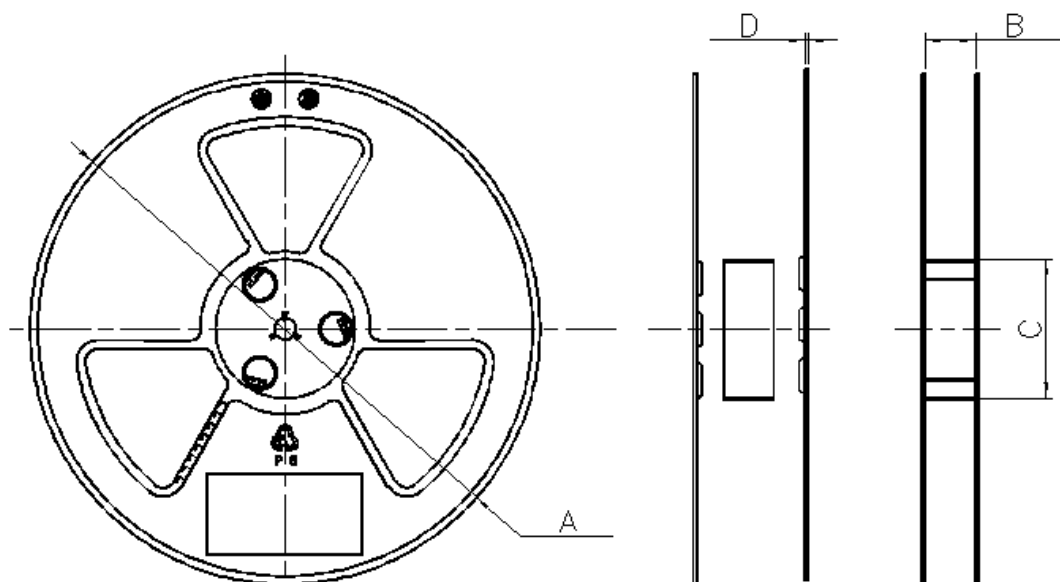
Figure 8-4. Reel Drawing for 13 Inch Reel
