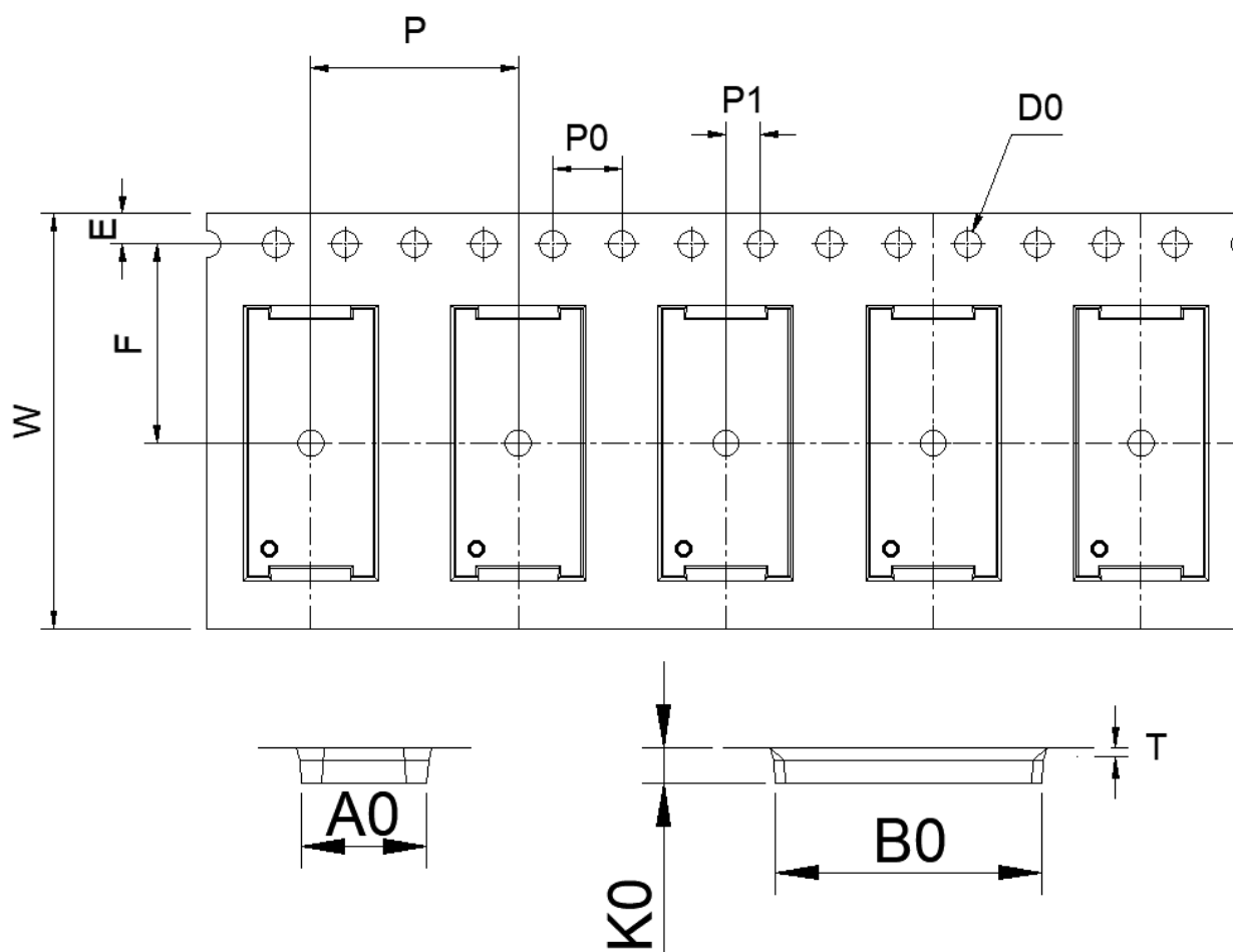
Figure 8-3. Tape and Reel Drawing for 13 Inch Reel
