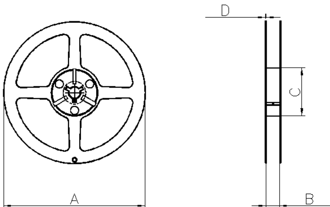
Figure 8-2. Reel Drawing for 7 Inch Reel
