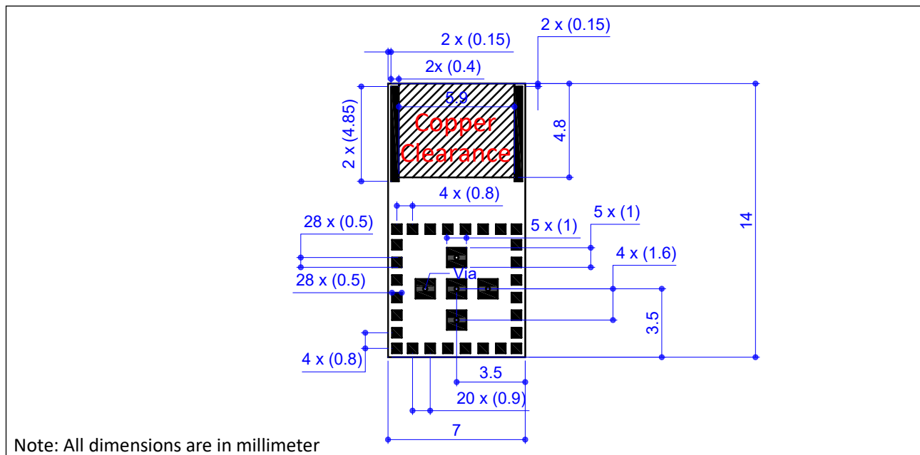
Figure 4-2. Module Footprint Top View
