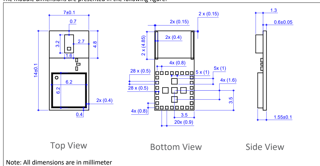
Figure 4-1. Mechanical Drawing
