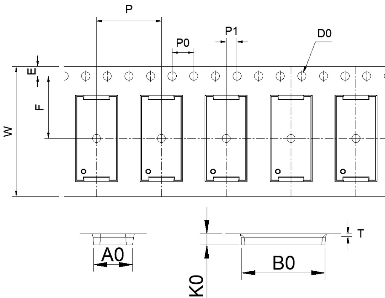
Figure 8-1. Tape and Reel Drawing for 7 Inch Reel
