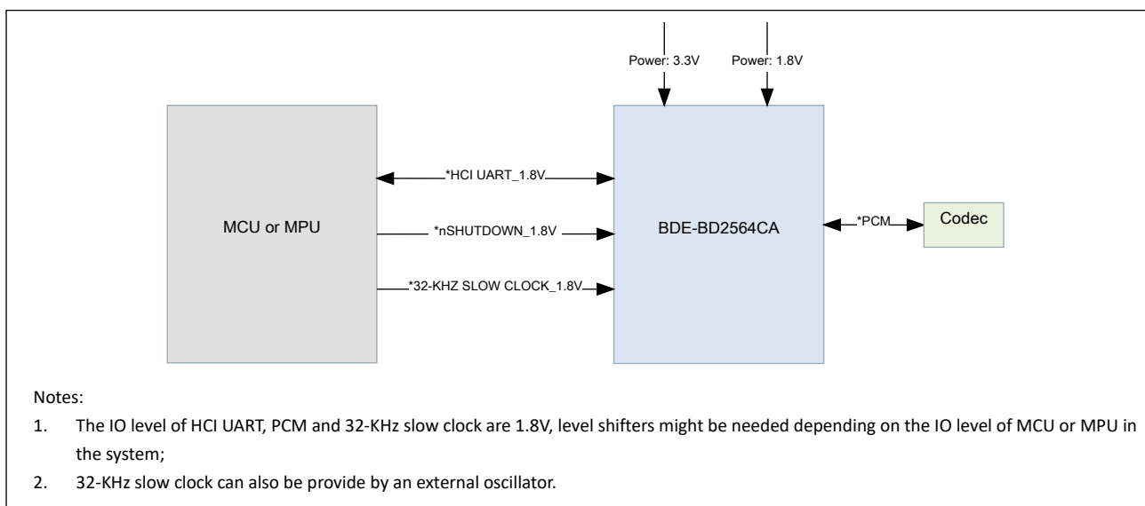
Figure 6-1. High-Level System Block Diagram
