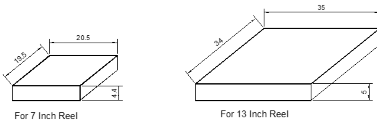
Figure 8-5. Reel Box Drawing
