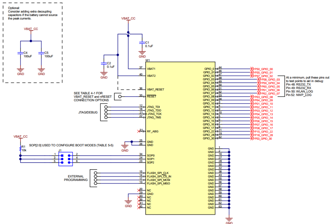
Figure 6-2. BDE-WF3235 Typical Application Schematic
