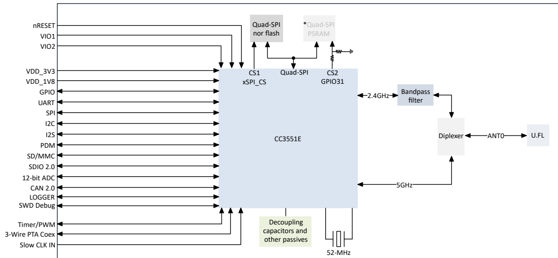
Figure 3. The Block Diagram of BDE-BW3551P1U
