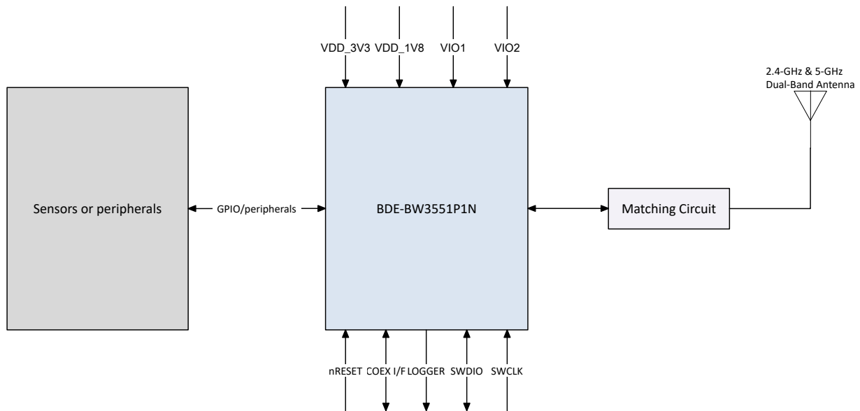
Figure 21. High-Level System Block Diagram
