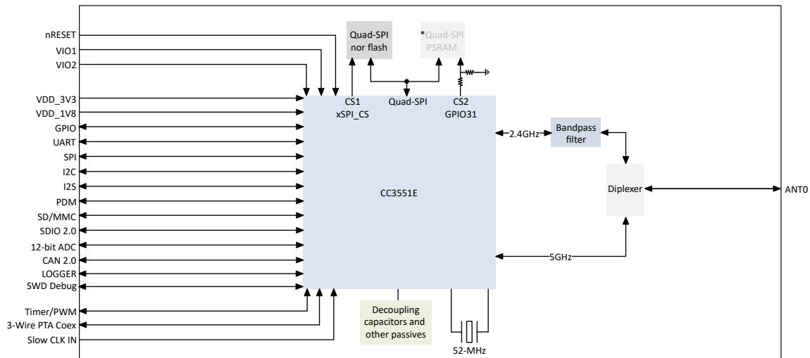
Figure 4. The Block Diagram of BDE-BW3551P1N
