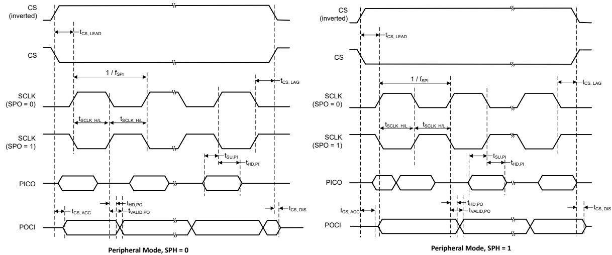
Figure 11. SPI Timing Diagrams - Peripheral Mode
