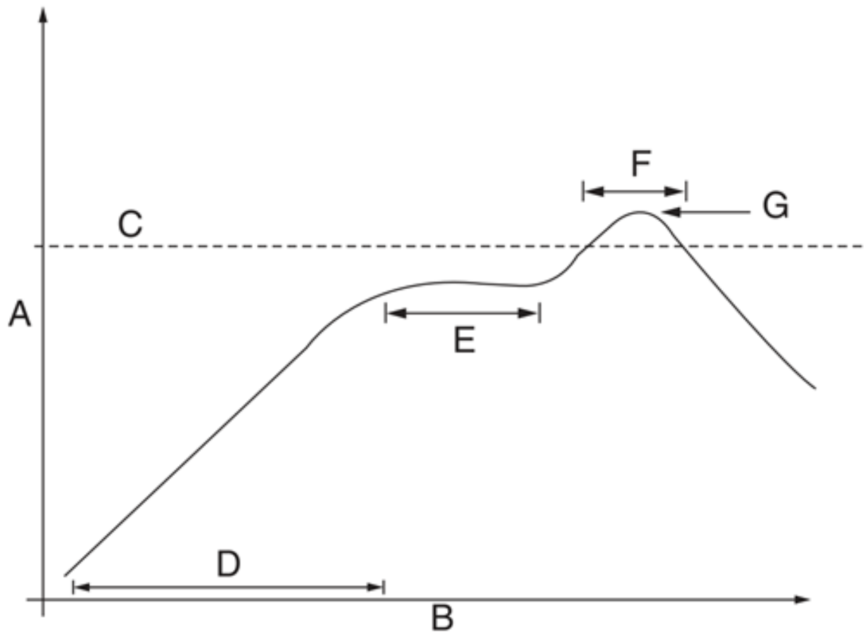
Figure 27. Thermal Profile Schematic
