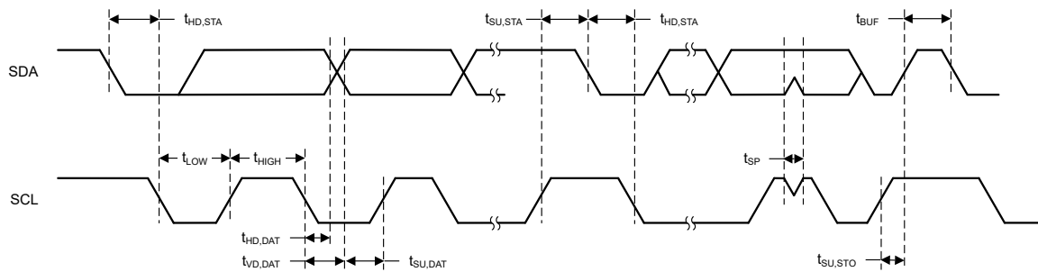
Figure 9. I2C Timing Diagram
