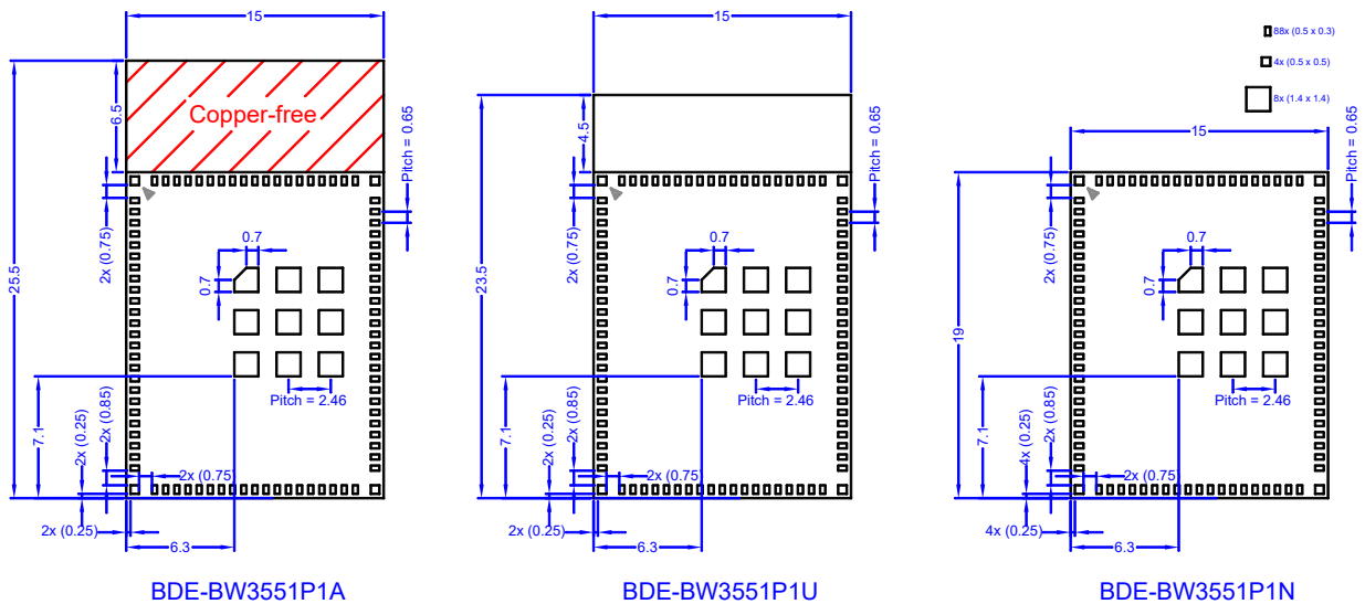
Figure 19. Recommended PCB Footprints
