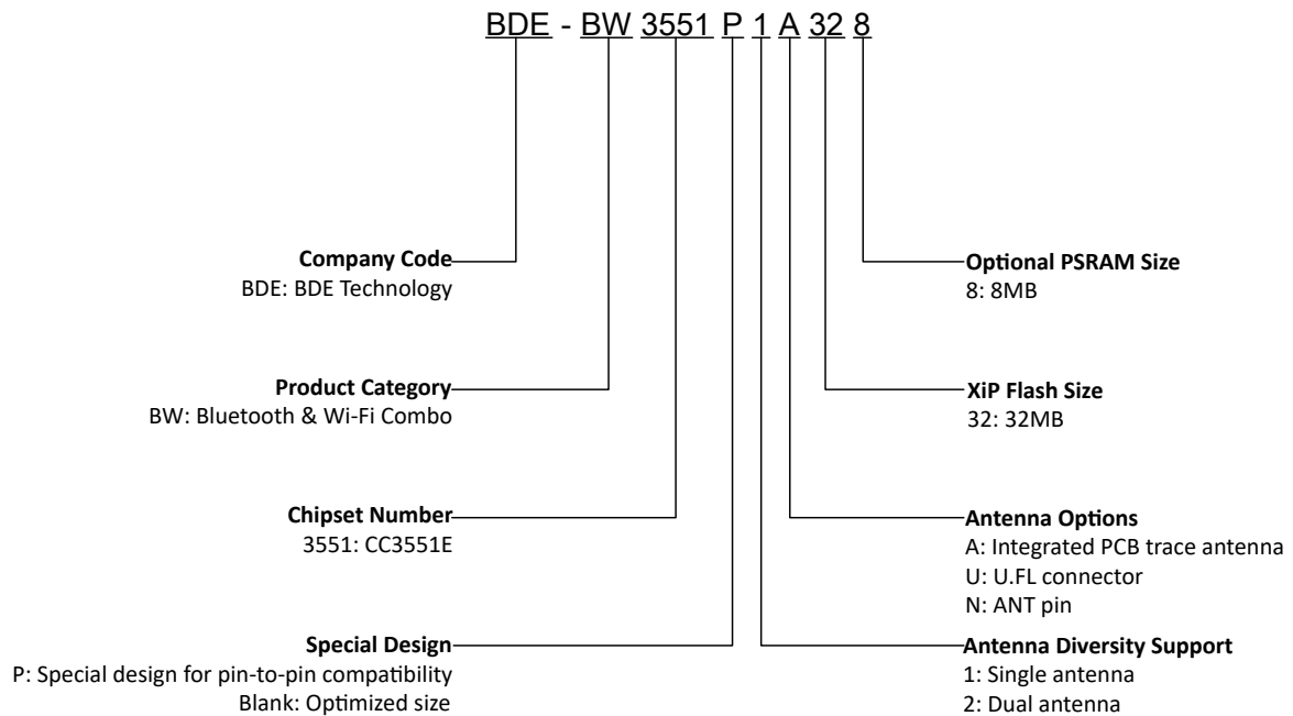
Figure 1. Naming Convention of Module Variants
