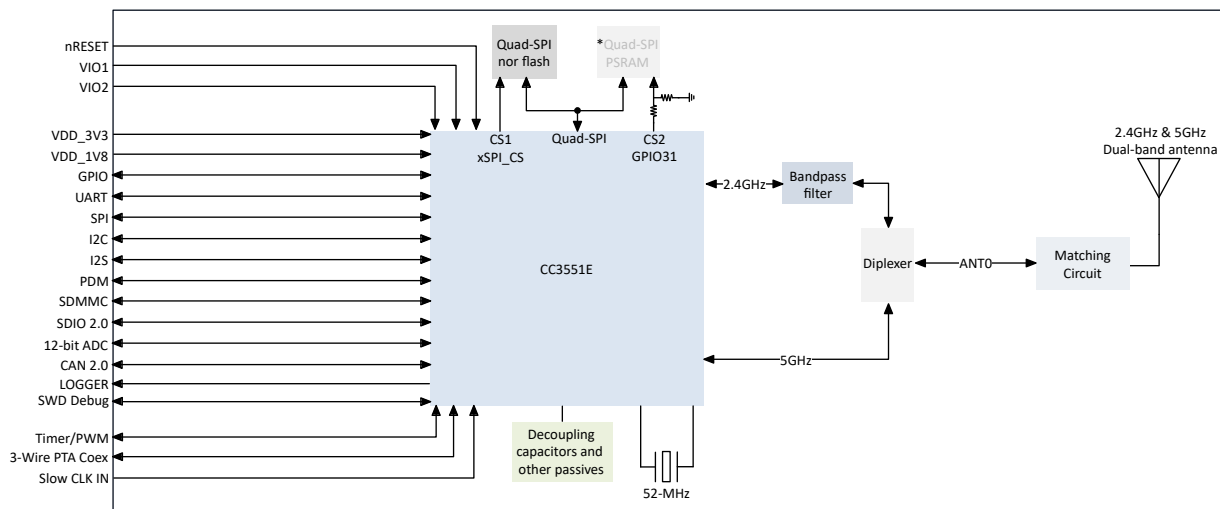
Figure 2. The Block Diagram of BDE-BW3551P1A
