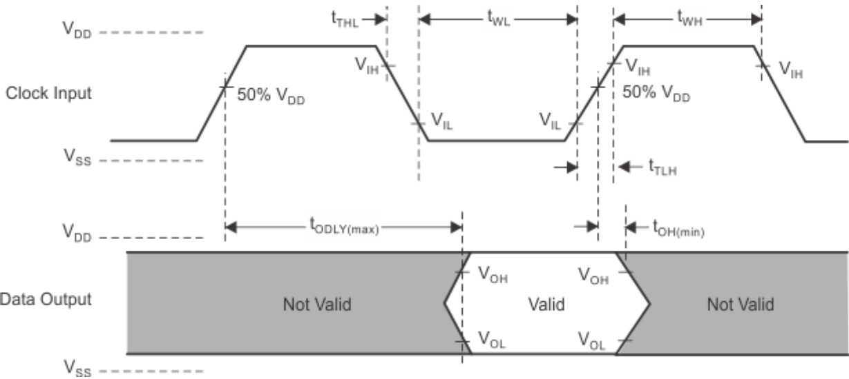
Figure 15. SDIO High Speed Output Timing
