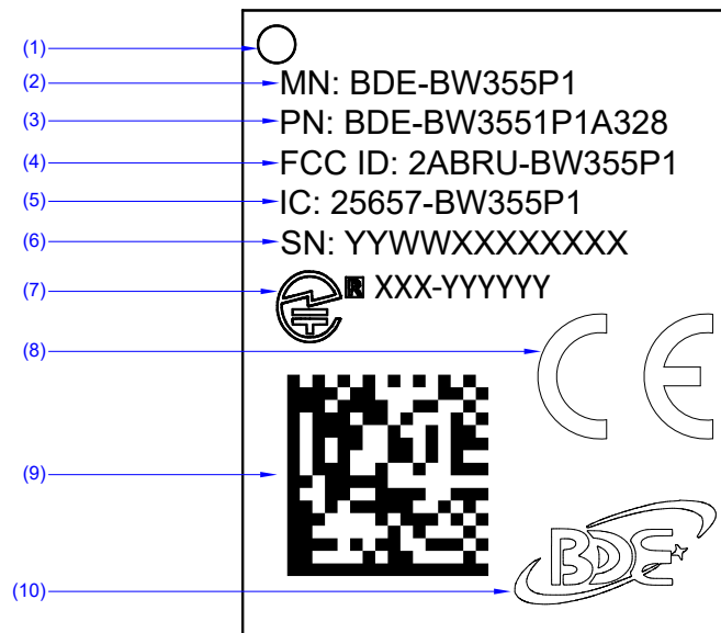
Figure 23. Module Marking
