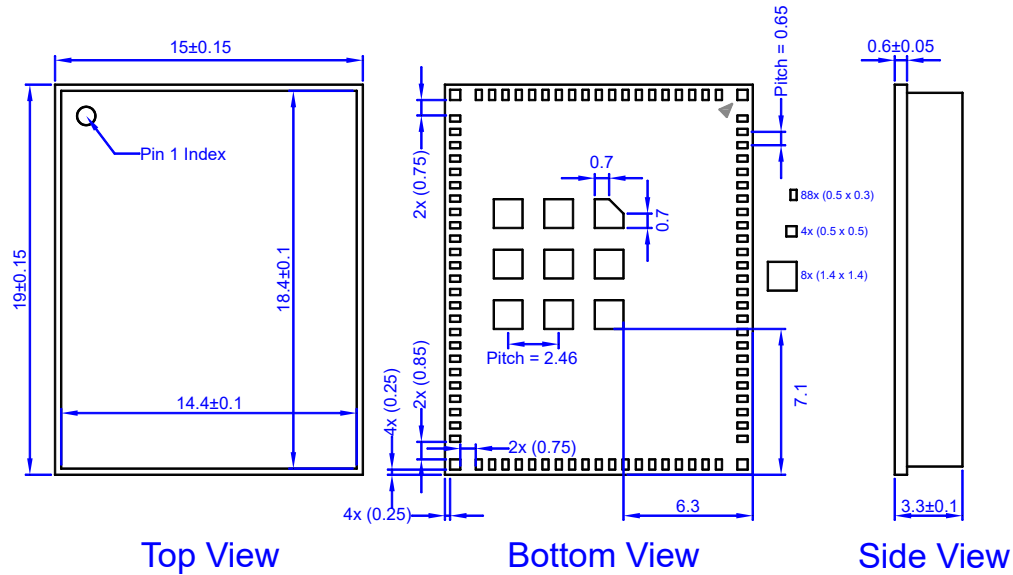
Figure 18. Mechanical Drawing of BDE-BW3551P1N
