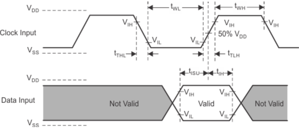
Figure 14. SDIO High Speed Input Timing
