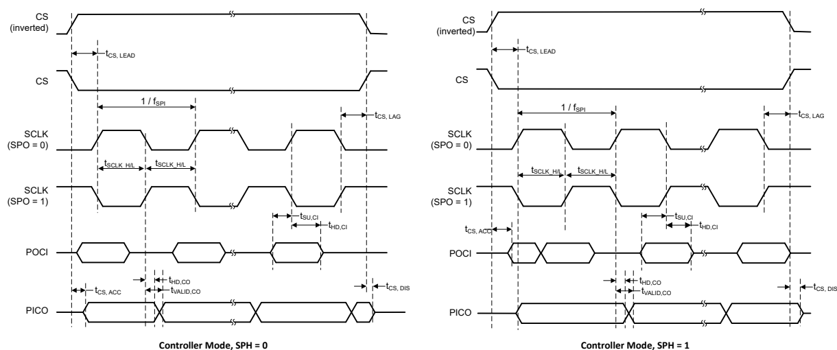
Figure 10. SPI Timing Diagrams - Controller Mode
