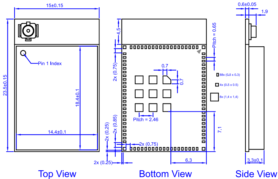
Figure 17. Mechanical Drawing of BDE-BW3551P1U
