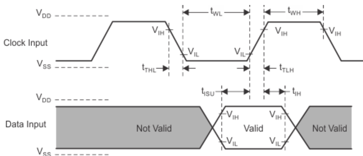
Figure 12. SDIO Default Input Timing
