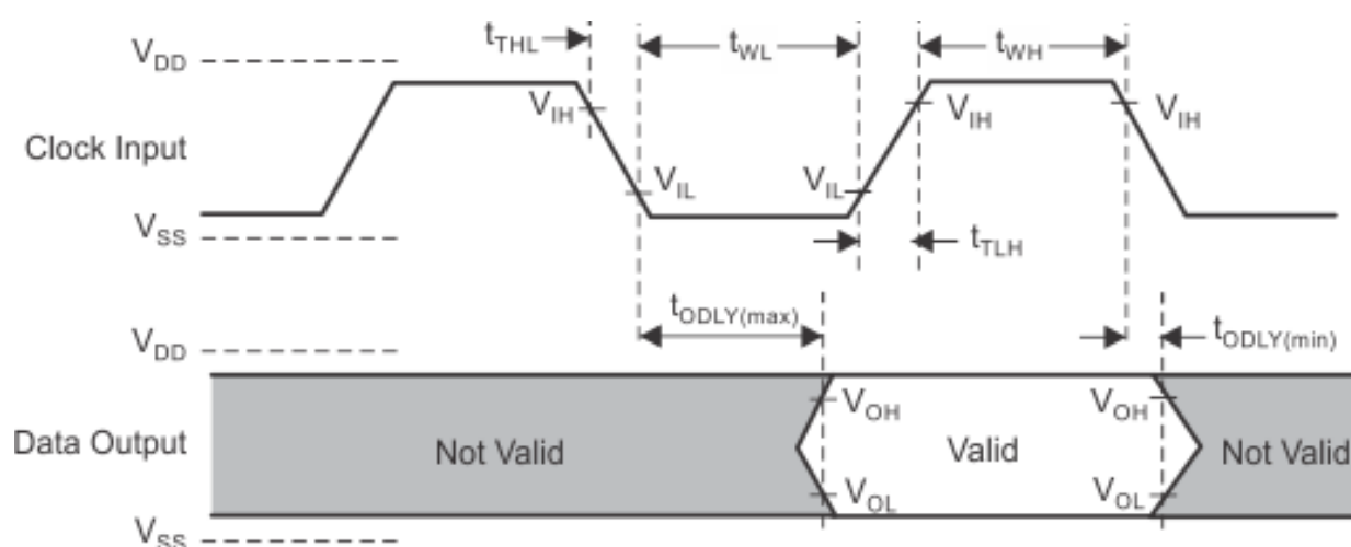
Figure 13. SDIO Default Output Timing
