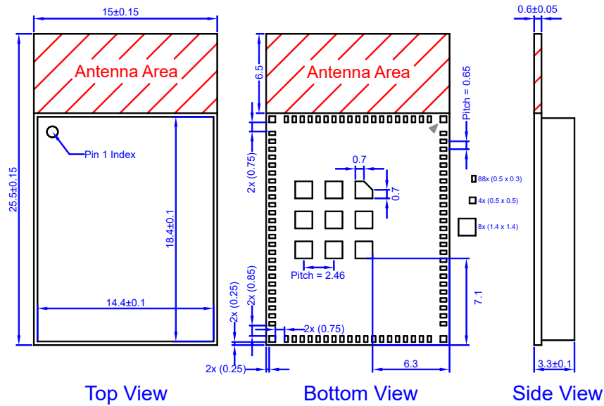
Figure 16. Mechanical Drawing of BDE-BW3551P1A
