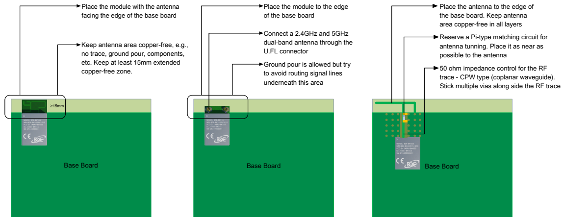
Figure 22. Recommended Module Placement
