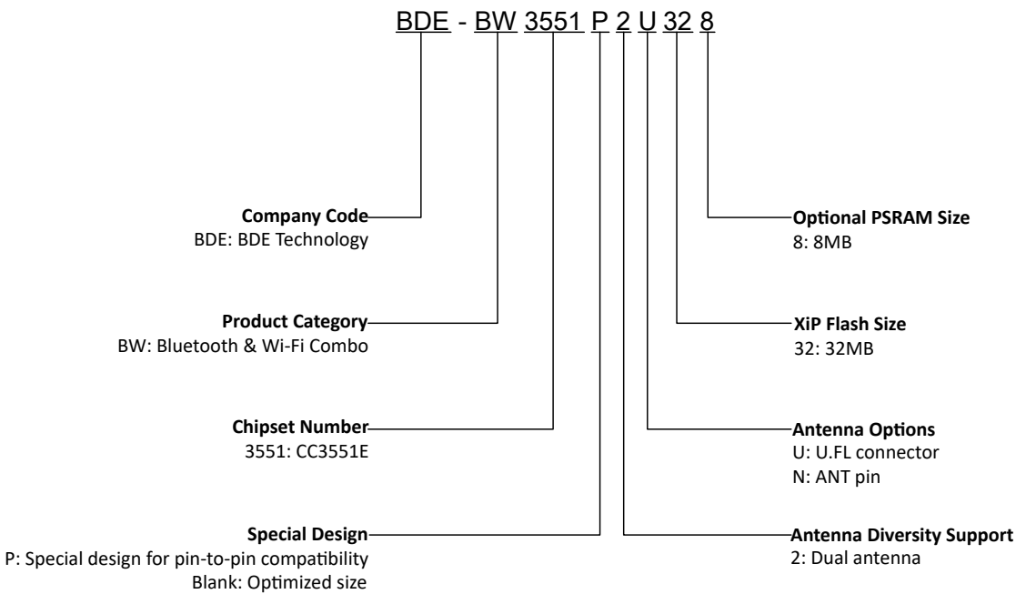
Figure 1. Naming Convention of Module Variants
