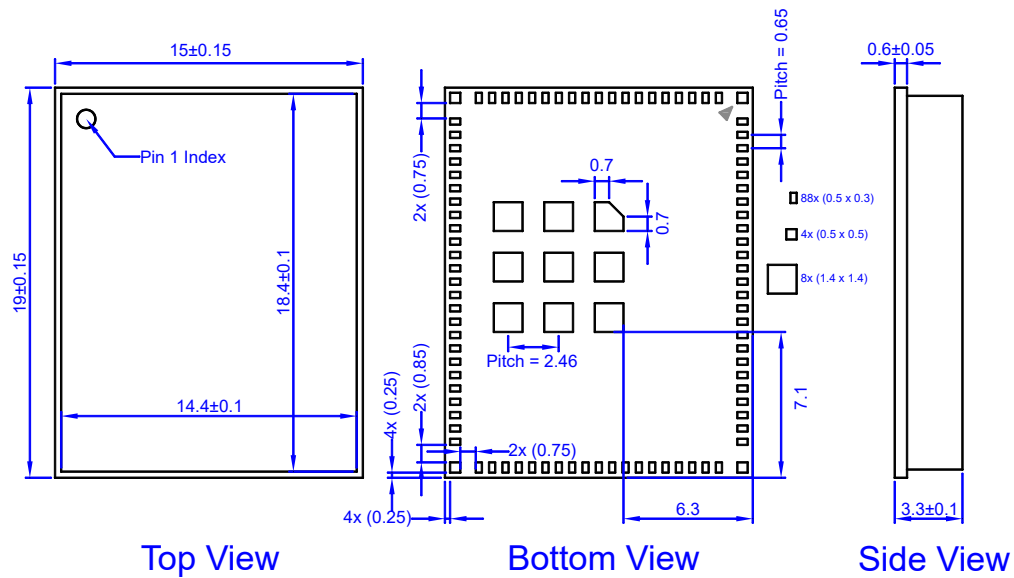
Figure 15. Mechanical Drawing of BDE-BW3551P2N
