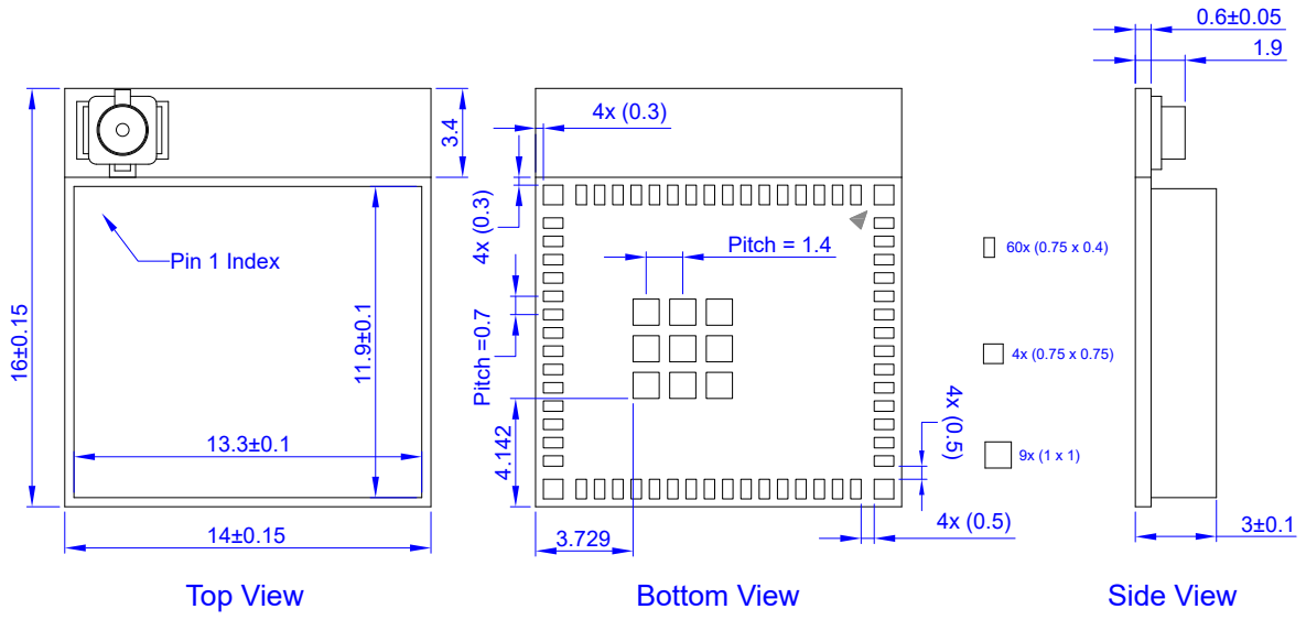
Figure 15. Mechanical Drawing of BDE-BW3551U
