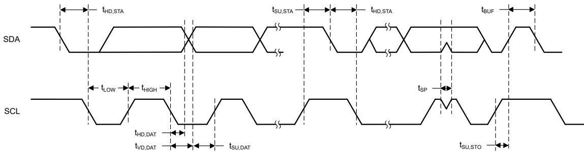
Figure 7. I2C Timing Diagram
