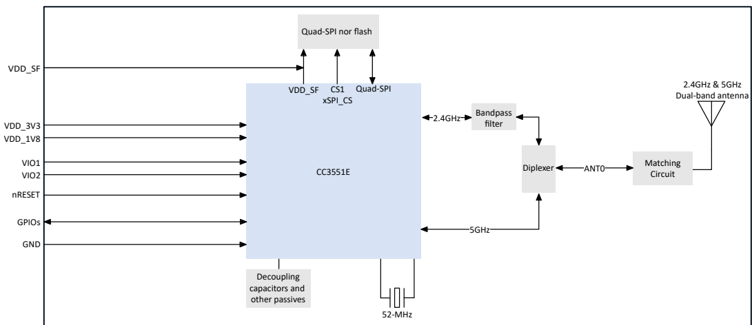
Figure 2. The Block Diagram of BDE-BW3551A Variants
