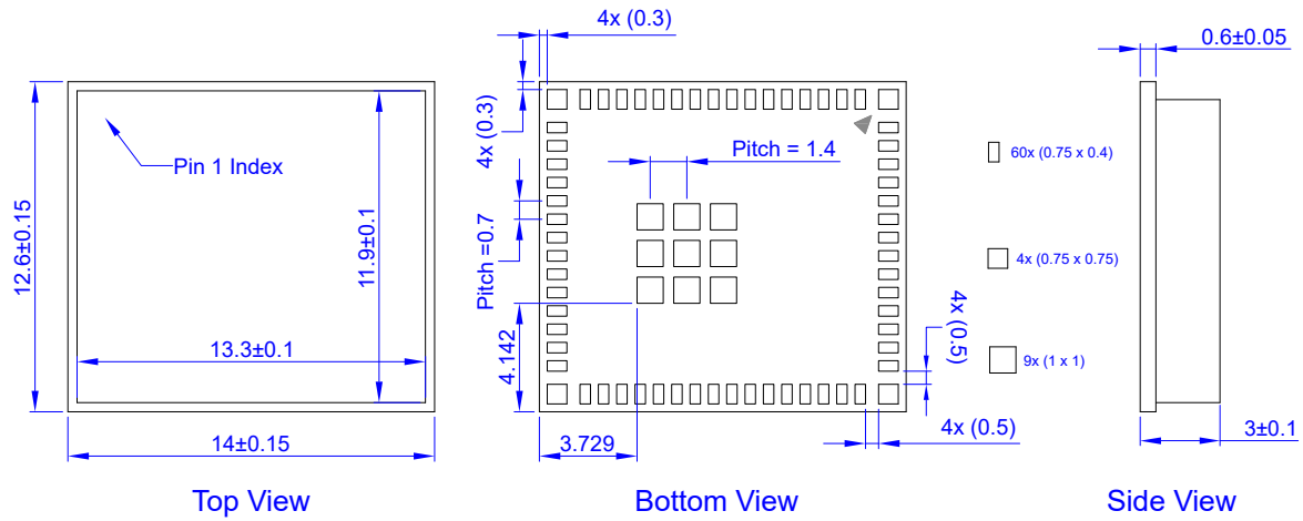
Figure 16. Mechanical Drawing of BDE-BW3551N
