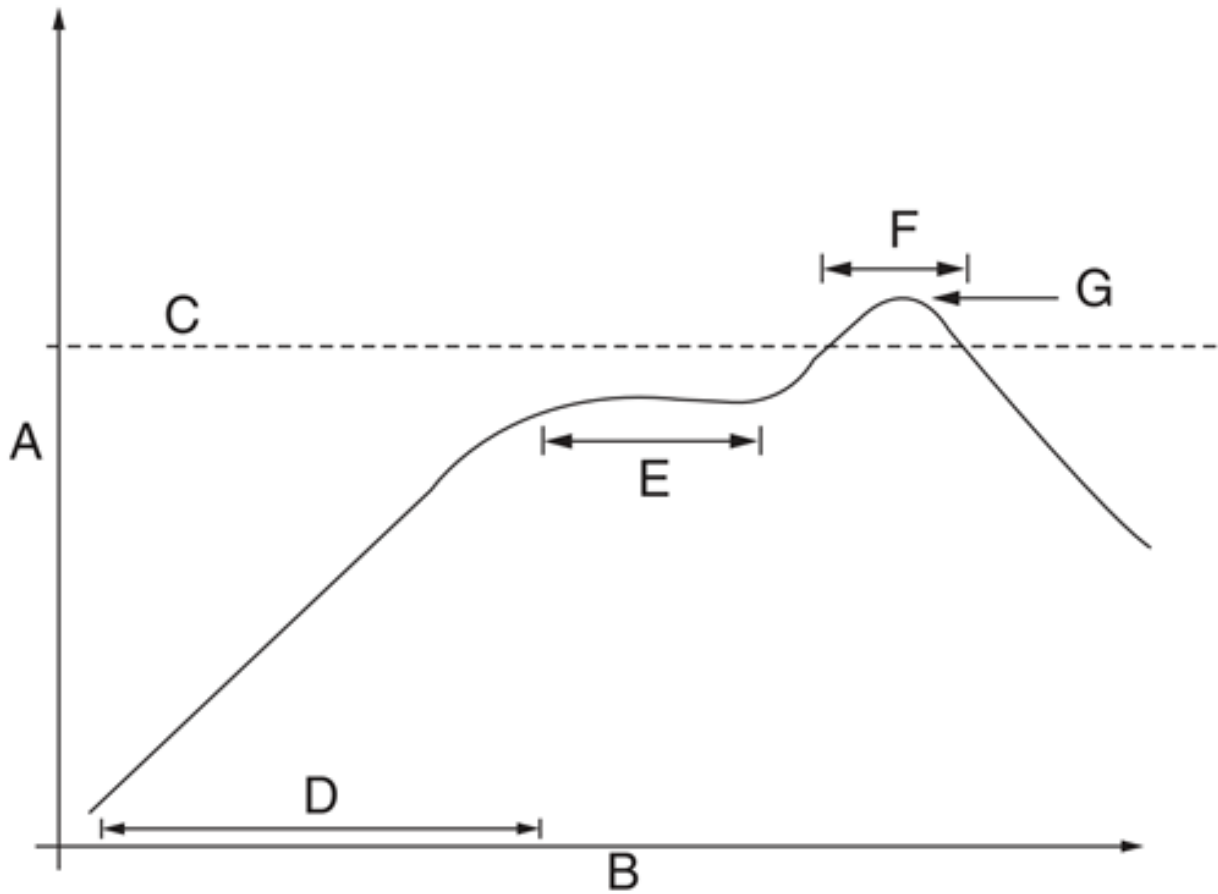
Figure 25. Thermal Profile Schematic
