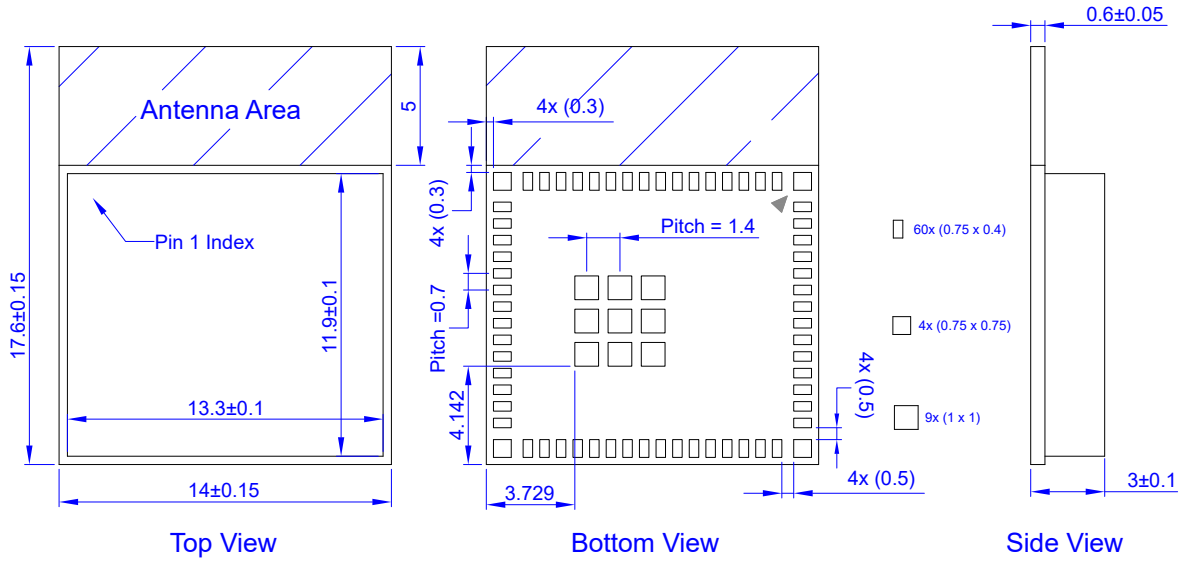
Figure 14. Mechanical Drawing of BDE-BW3551A
