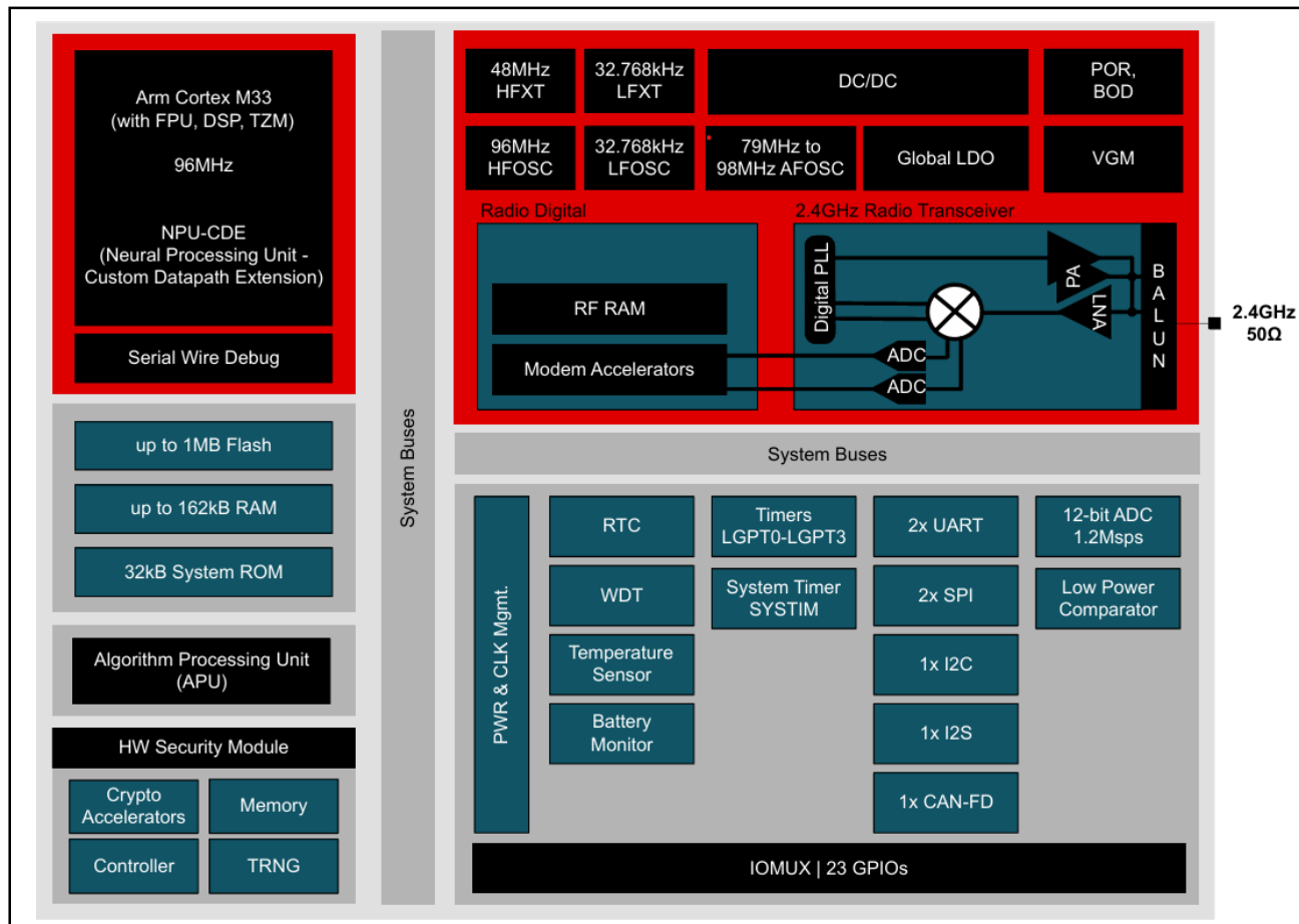
Figure 3. The block diagram of CC2755P10 (Adopted from CC2755P10 datasheet)
