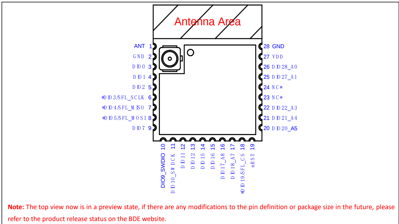
Figure 4. Pinout Diagram of BDE-MP2755P10 Top View
